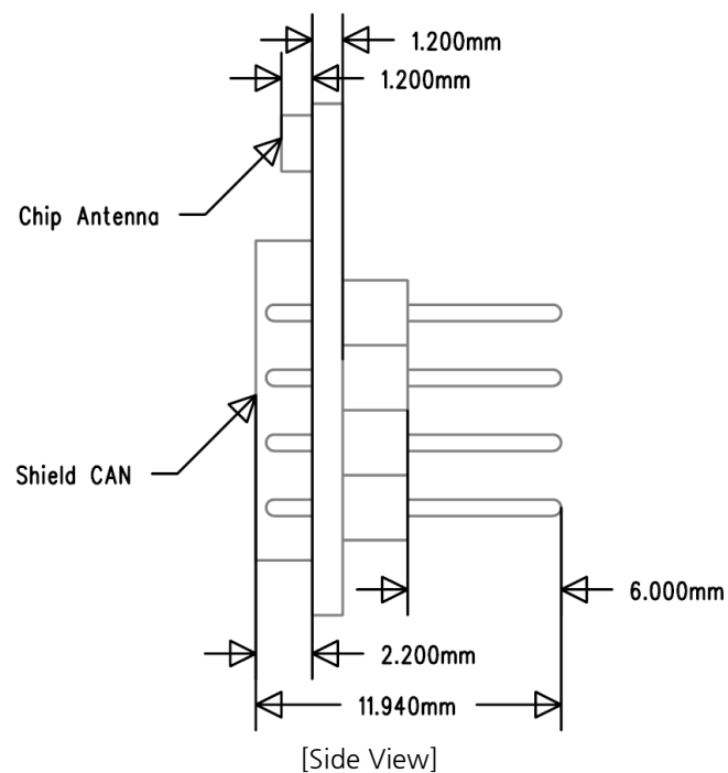
<Figure 4-1 FBL700BC Dimension>
