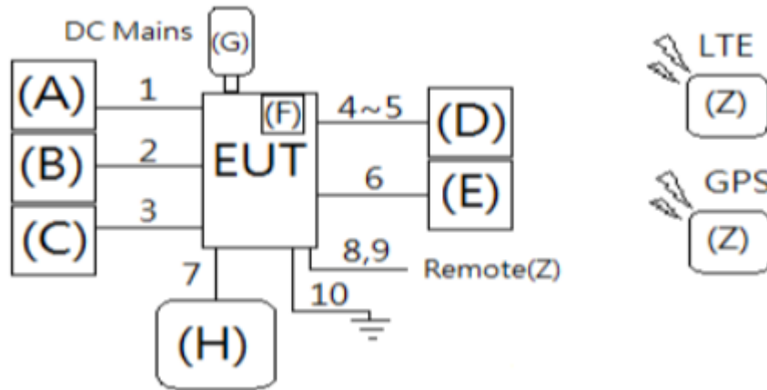
Test Setup Diagram (Conducted emission and radiated emission below 1GHz)
