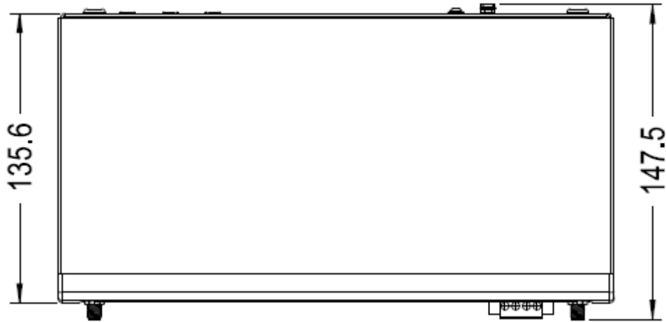
Front view
