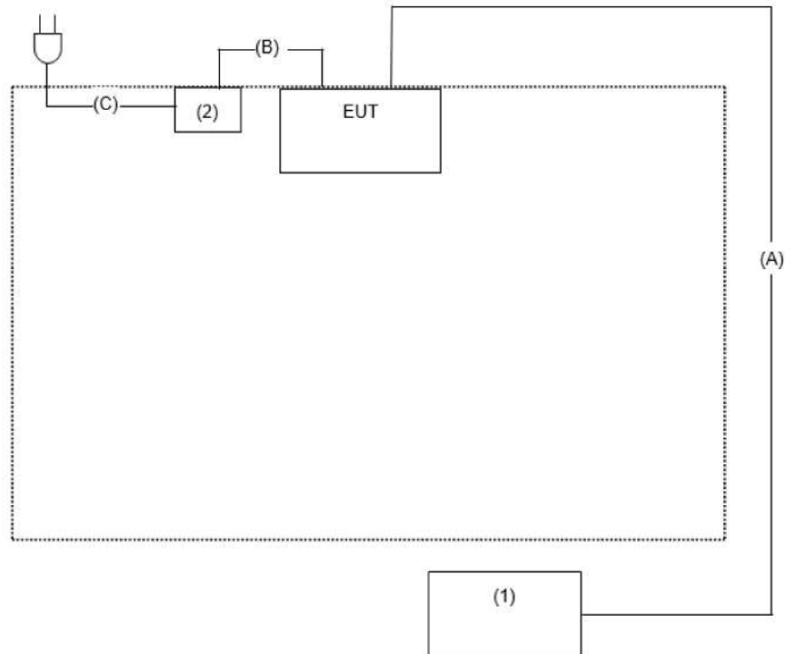
Connection Diagram - Power by 802.03at PoE
