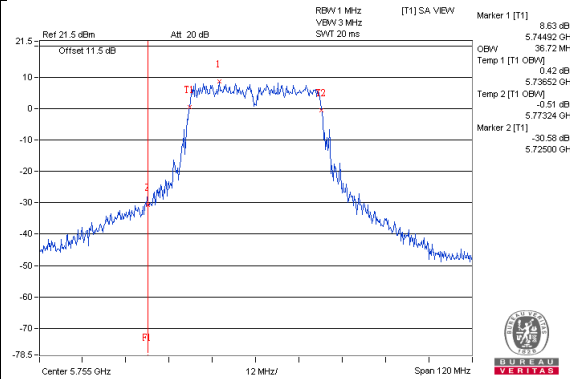
802.11ac(VHT40)_Chain1 / CH151
