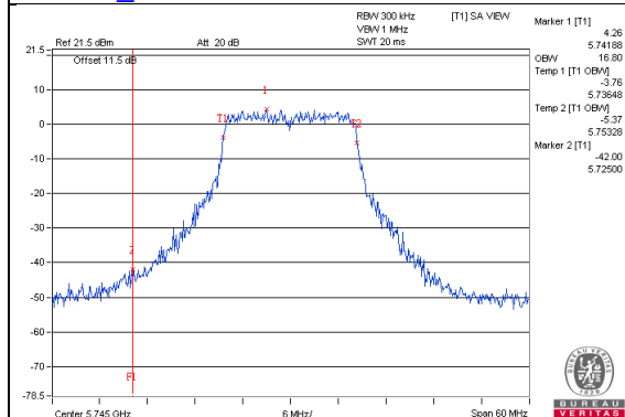
802.11ac(VHT20)_Chain0 / CH149
