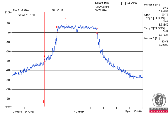
802.11ac(VHT40)_Chain1 / CH151
