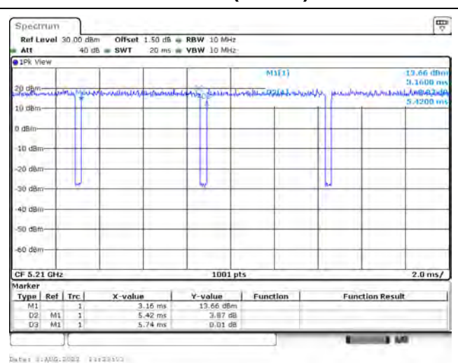
802.11ax (80 MHz)
