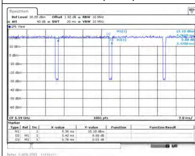
802.11ax (40 MHz)
