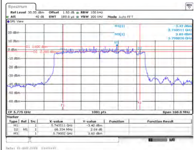
802.11ax (80 MHz) / Ant. 1 / 5775 MHz
