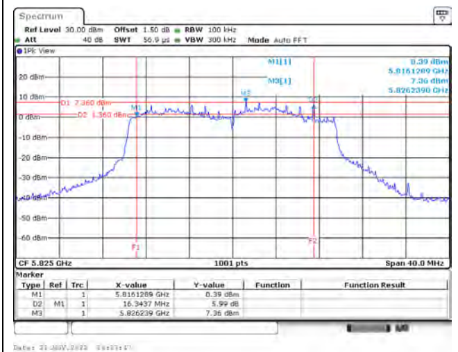
802.11ax (20 MHz) / Ant. 1 / 5825 MHz
