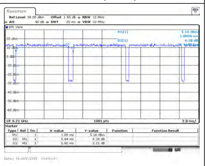
802.11ax (80 MHz)
