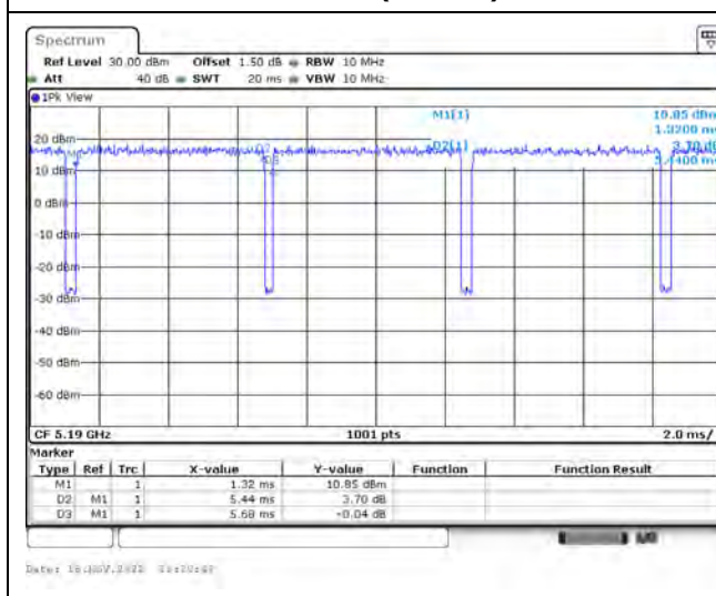
802.11ax (40 MHz)
