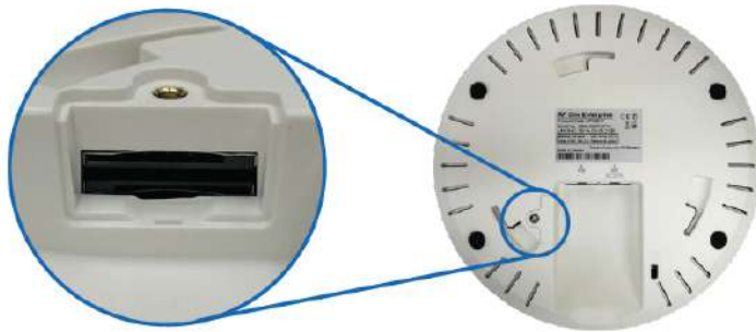
Screw Open the Panel to Reveal Redundant SIM Slots
