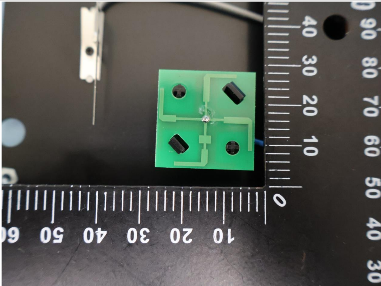
Antenna 12
