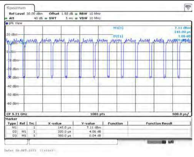
802.11ac (80 MHz)
