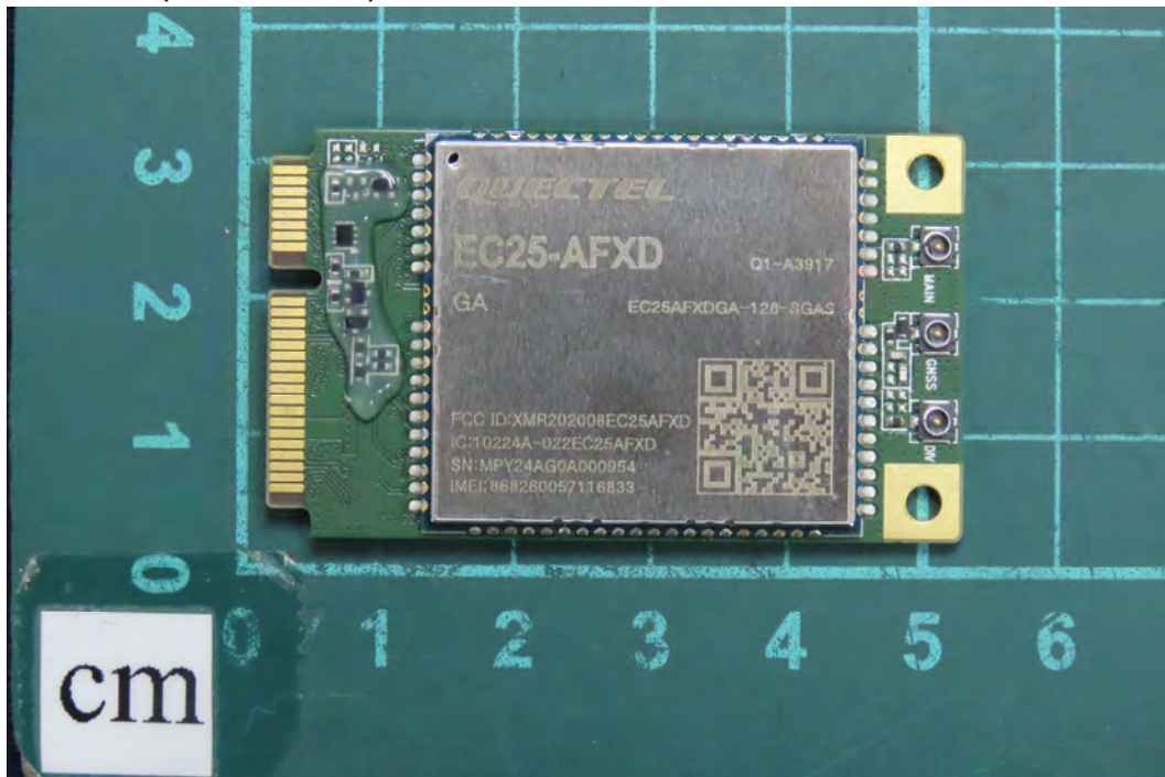
(8) EUT Photo (WWAN Module)
