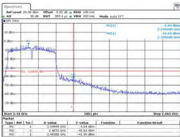
802.11ac40 / Chain A / 2452 MHz (Band Edge)
