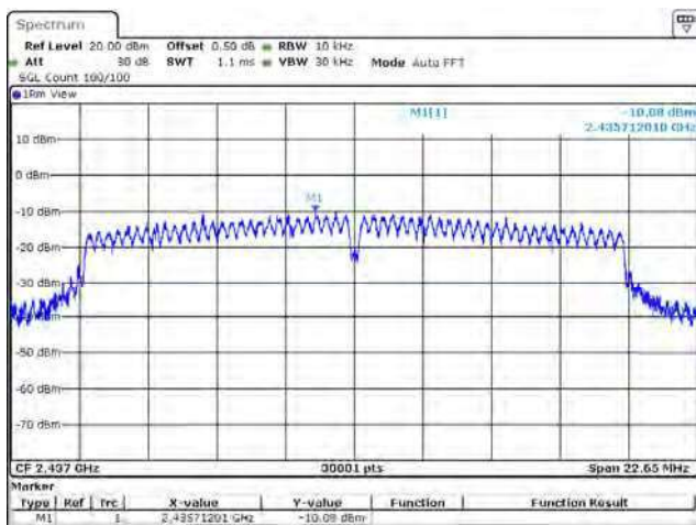
802.11ac (20 MHz) / Chain A / 2437 MHz
