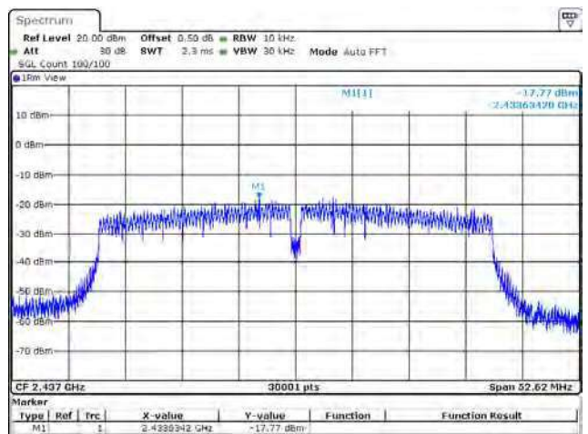
802.11ac (40 MHz) / Chain B / 2437 MHz
