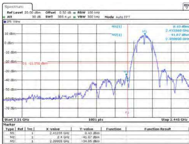
802.11b / Chain A / 2412 MHz (Band Edge)
