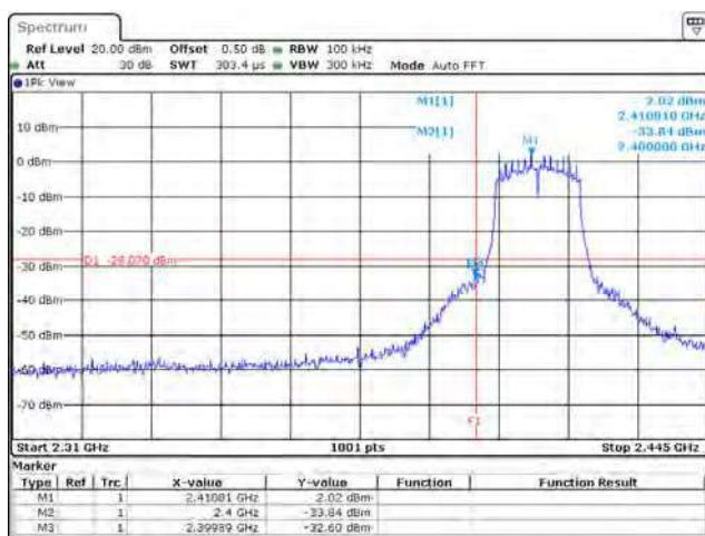
802.11g / Chain A / 6M 2412 MHz (Band Edge)
