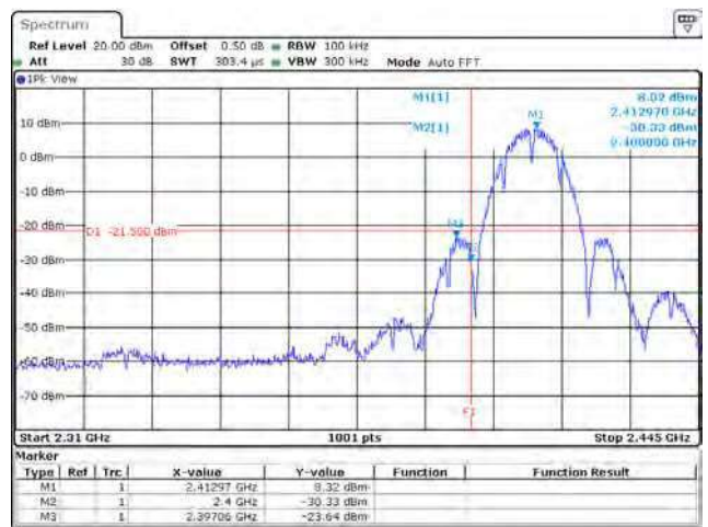
802.11b / Chain B / 2412 MHz (Band Edge)
