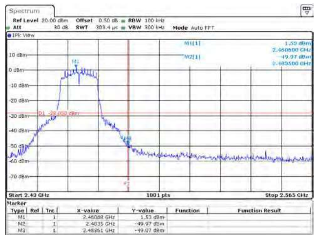
802.11g / Chain B / 2462 MHz (Band Edge)
