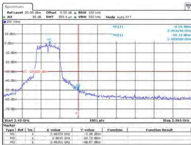
802.11g / Chain A / 2462 MHz (Band Edge)
