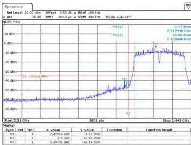
802.11ac40 / Chain A / 2422 MHz (Band Edge)
