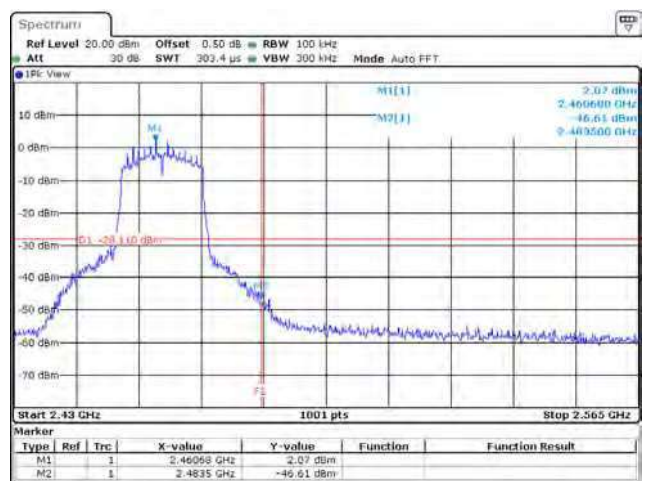
802.11ac20 / Chain B / 2462 MHz (Band Edge)
