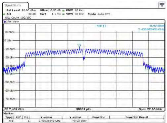
802.11g / Chain A / 2437 MHz
