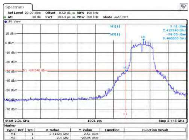
802.11g / Chain B / 6M 2412 MHz (Band Edge)
