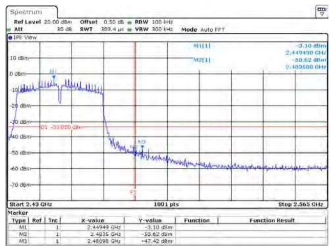
802.11ac40 / Chain B / 2452 MHz (Band Edge)
