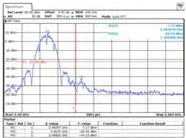
802.11b / Chain B / 2462 MHz (Band Edge)
