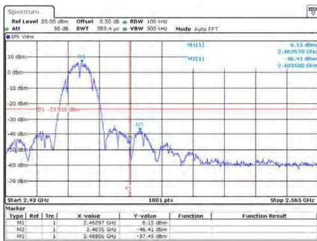
802.11b / Chain A / 2462 MHz (Band Edge)
