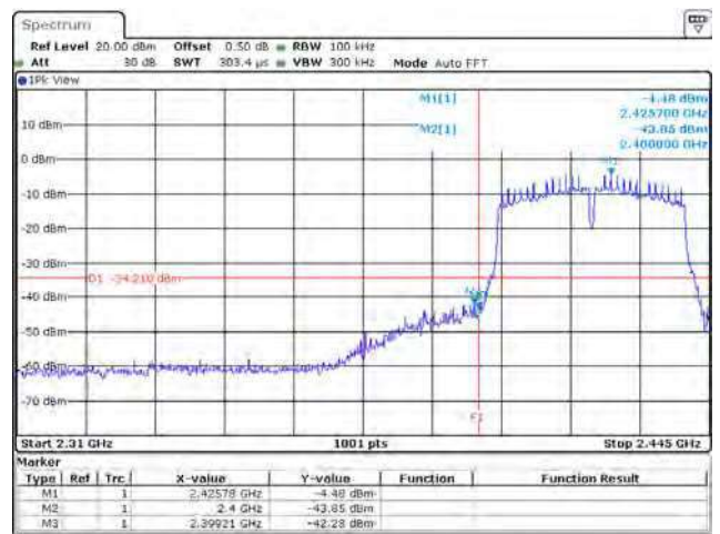
802.11ac40 / Chain B / 2422 MHz (Band Edge)
