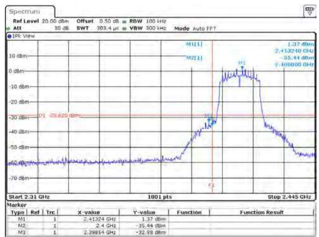
802.11ac20 / Chain B / 2412 MHz (Band Edge)
