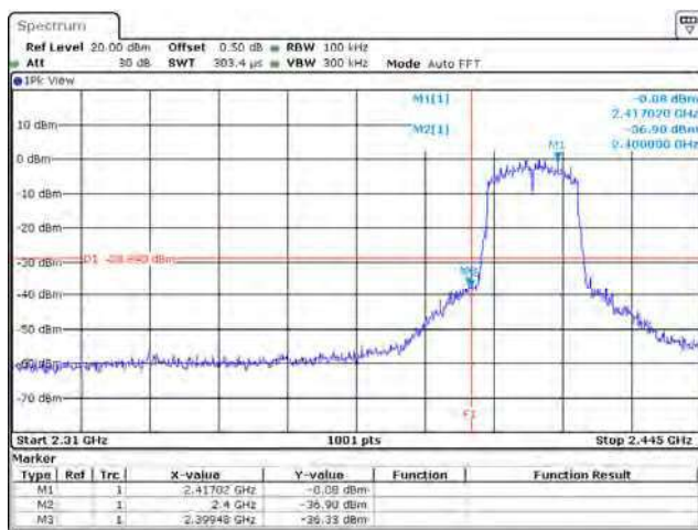
802.11ac20 / Chain A / 2412 MHz (Band Edge)
