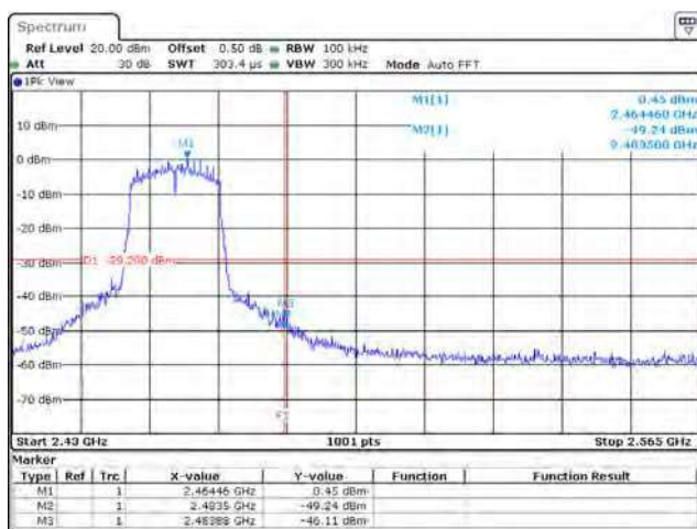
802.11ac20 / Chain A / 2462 MHz (Band Edge)
