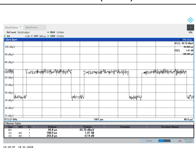
802.11ac (80 MHz)
