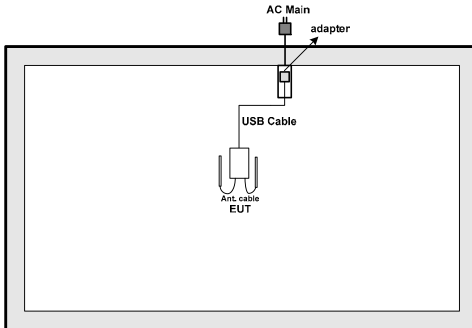
Test Setup Diagram - Radiated Emission Above 1GHz (Mode 1)
