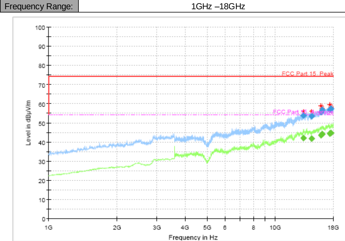
Mode 1: GSM1900 receiver +PA01+BA01&lt;Figure 1&gt;
