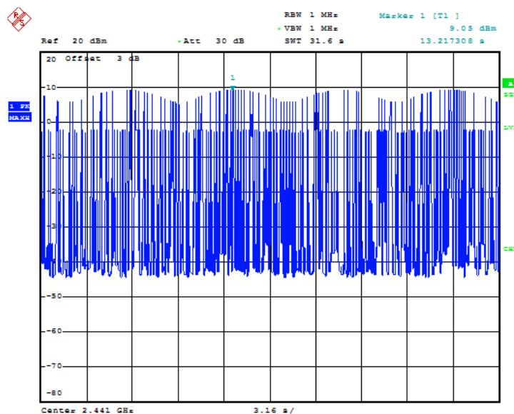
Fig.62 Time of occupancy (Dwell Time): Ch39,Packet 3-DH5
