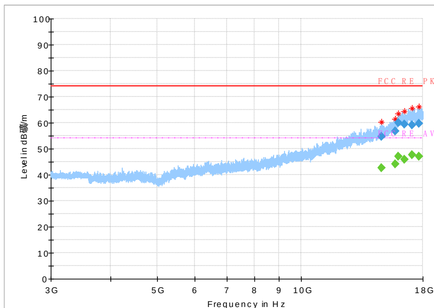
Fig.33 Radiated emission: GFSK, Ch0, 3GHz~18GHz
