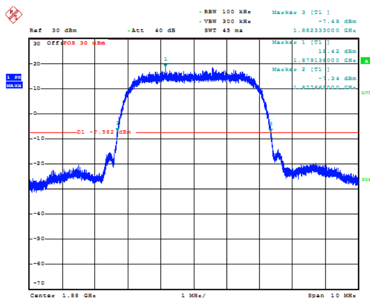
Fig.34 Channel 9262- Emission Bandwidth (-26dBc BW)
