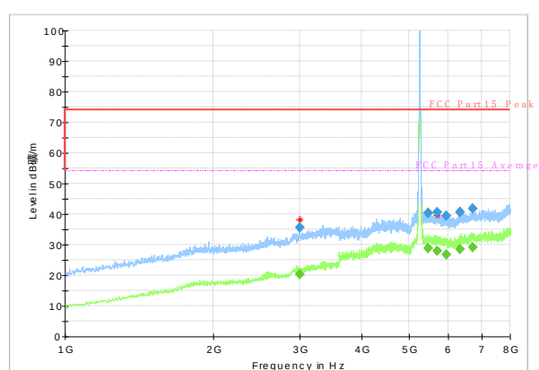
Radiated Spurious Emission (802.11ac-VHT20, ch48, 1GHz-8GHz)
