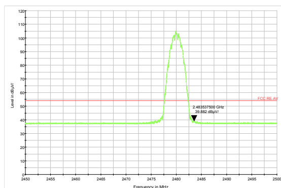
3DH5-Channel 78: Average
