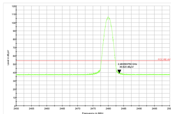
DH5-Channel 78: Average
