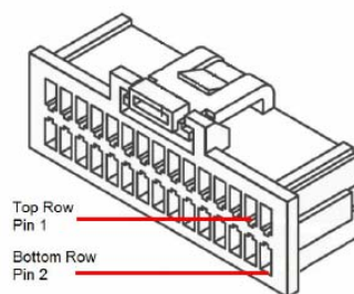
Figure 10: Main 20 pin connector
