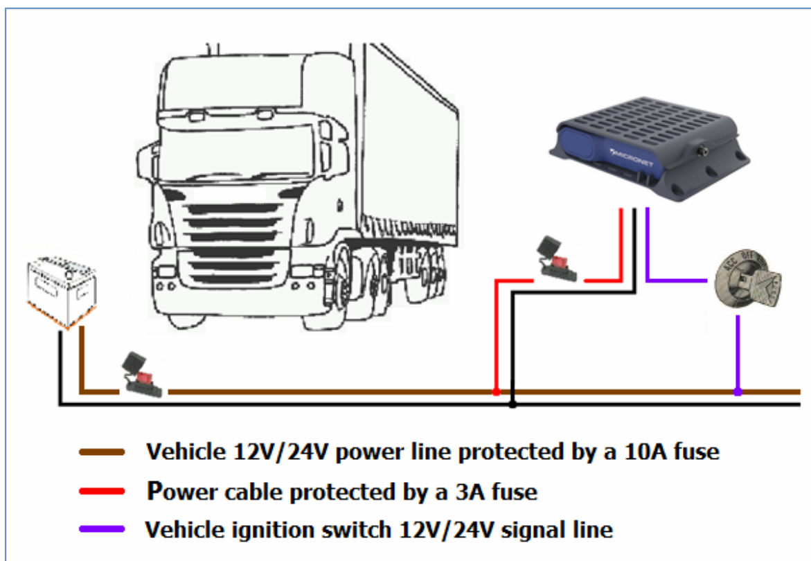
Figure 11: Electrical Installation Scheme
