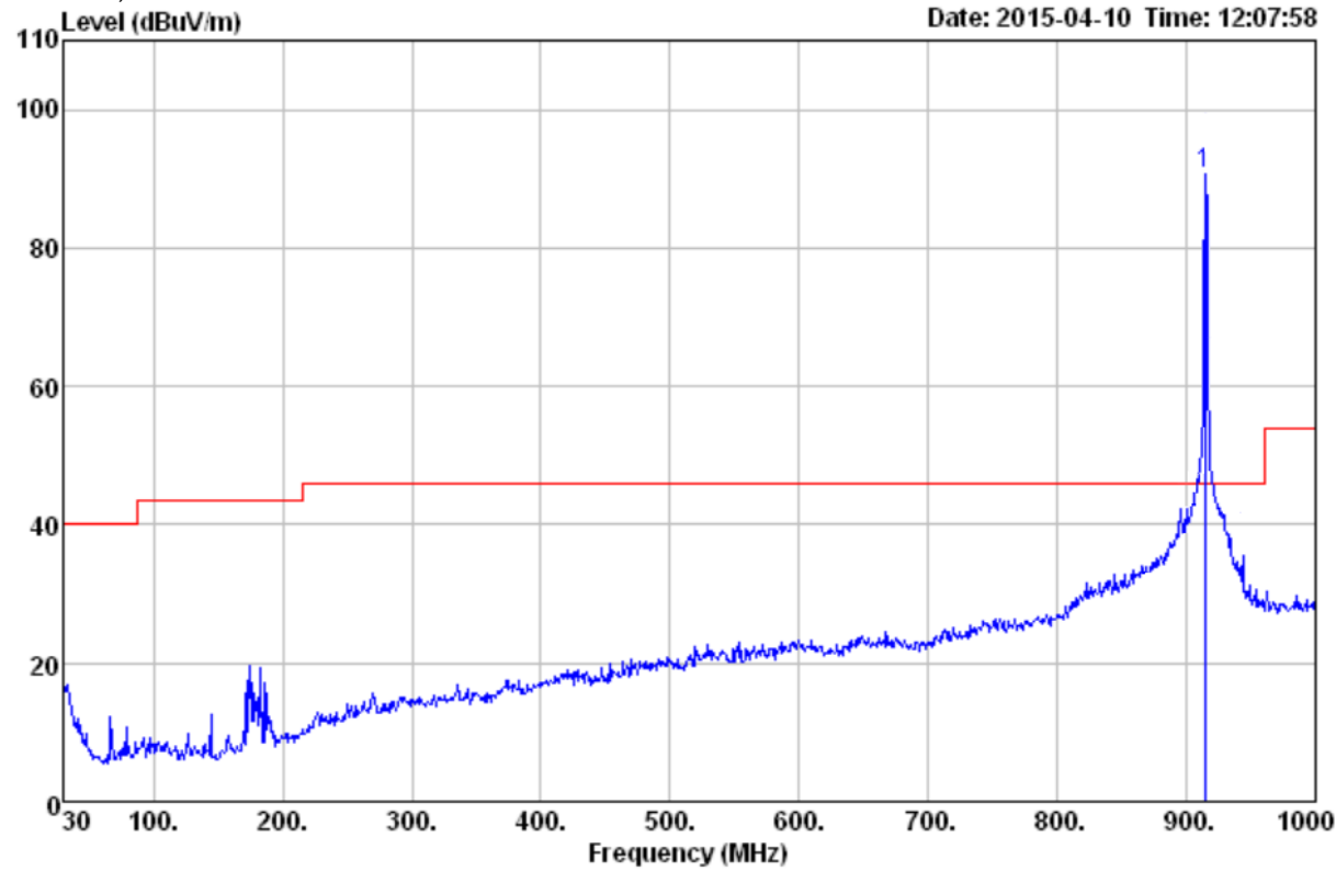
Quasi-peak measurement
