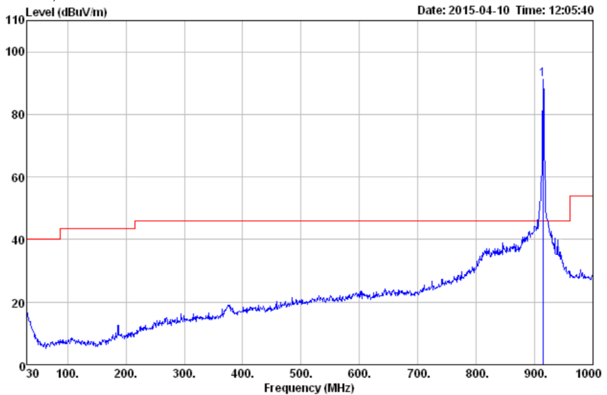
Quasi-peak measurement
