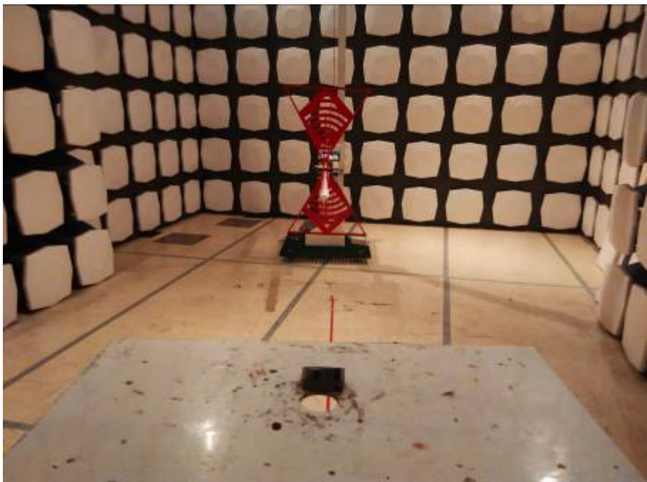
SIGNOLUXUTX-B: 30MHz – 1GHz
