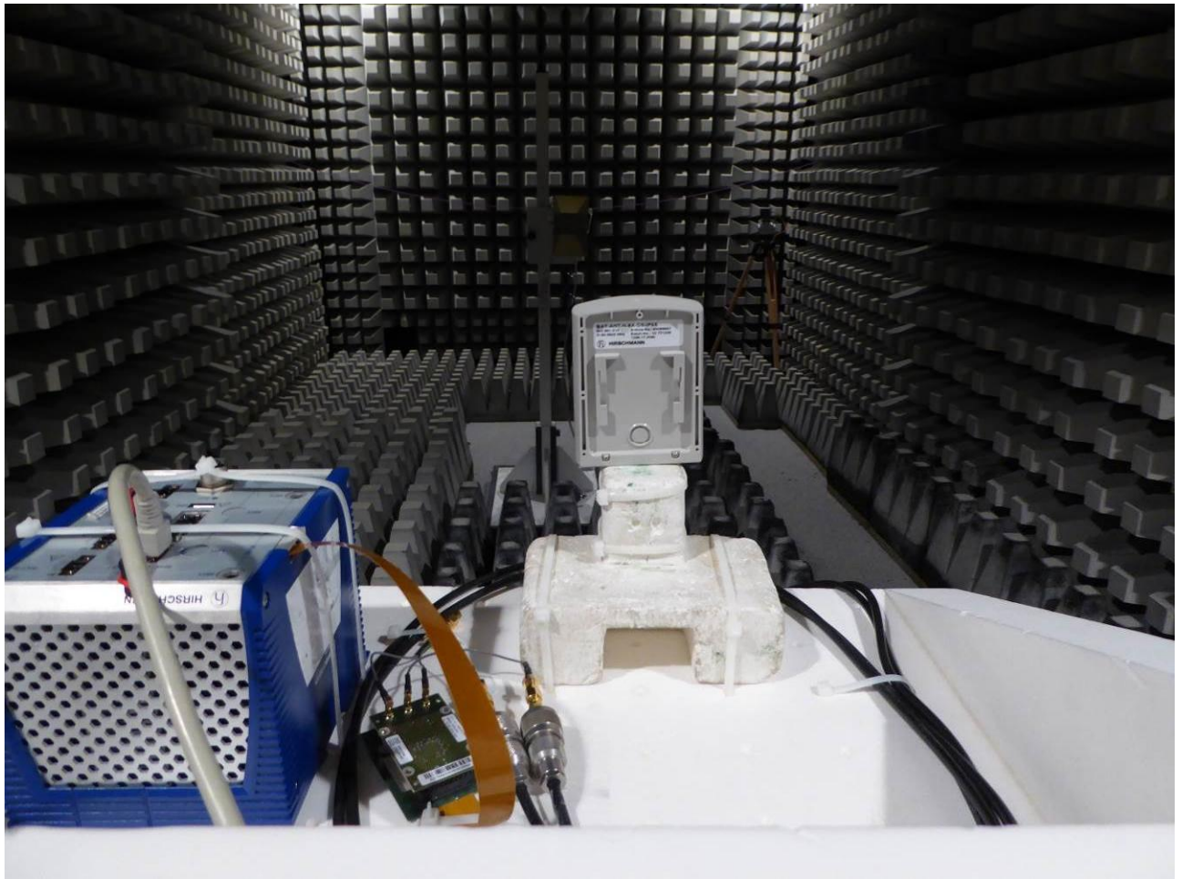
160307_03: Test setup - Radiated emission anechoic chamber, BAT-ANT-N-9A-DS-IP65 antenna
