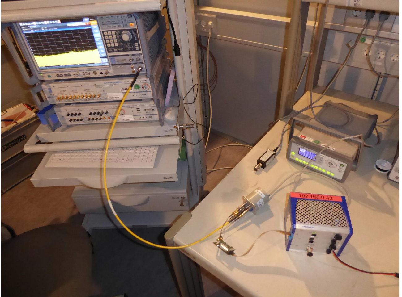
Test setup – conducted measurement
