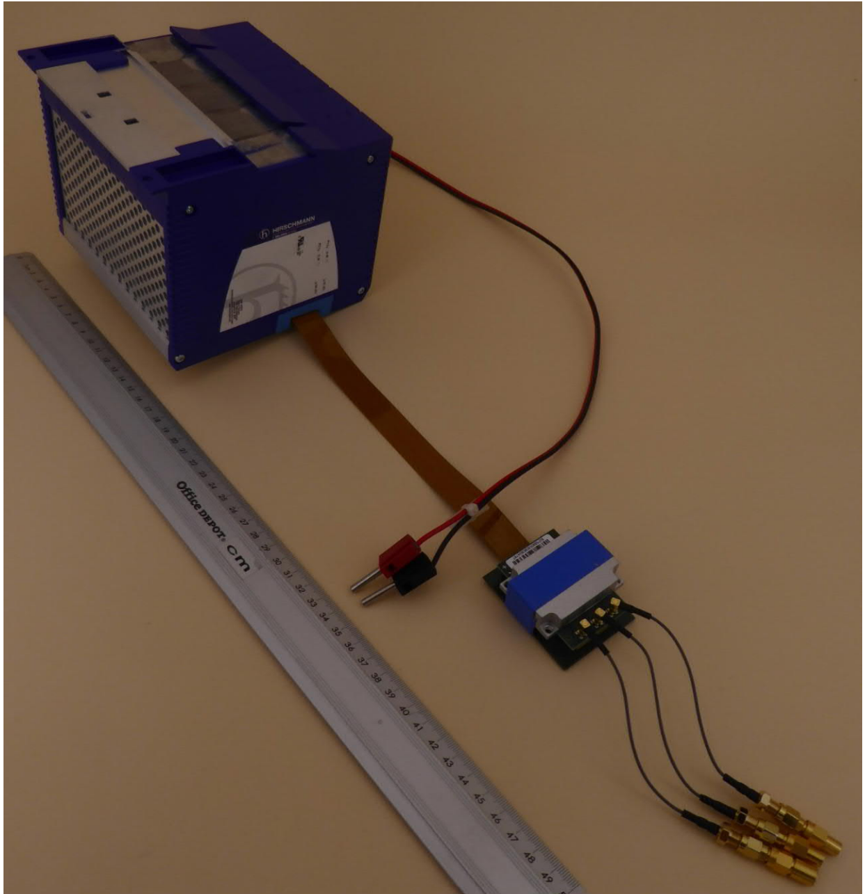
EUT with BAT-R host device – 3D view 2
