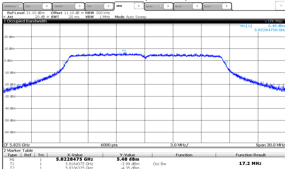
Channel 165 (5825 MHz)
