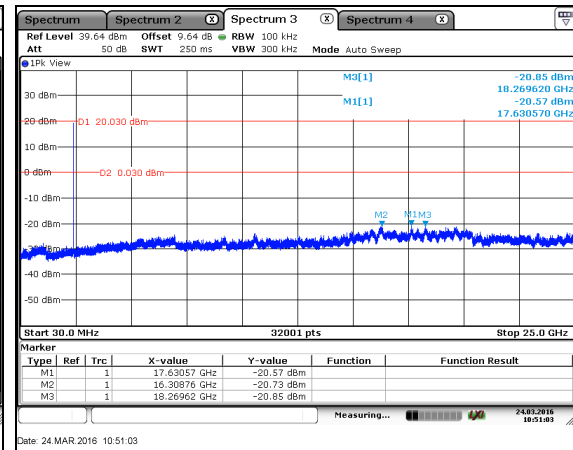
Figure 7.5.1.2-6: 30 MHz – 25 GHz – LCH – u.fl Port
