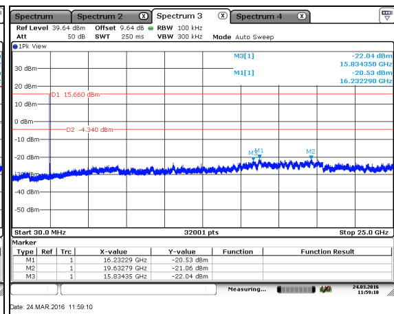
Figure 7.5.1.2-8: 30 MHz – 25 GHz – HCH – u.fl Port
