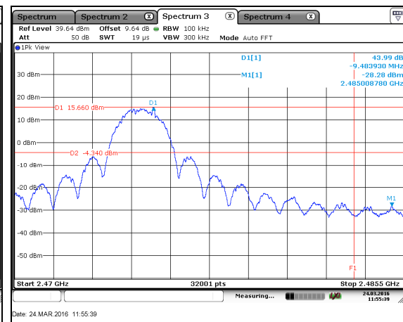
Figure 7.5.1.2-10: Upper Band-edge – HCH – u.fl Port
