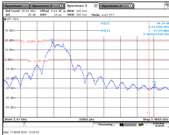
Figure 7.5.1.2-5: Upper Band-edge – HCH R-SMA Port
