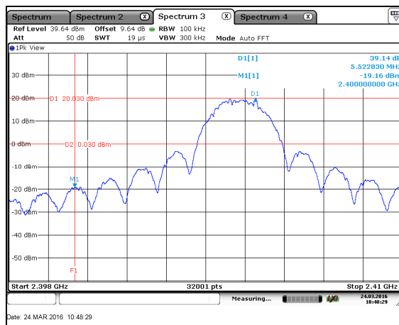
Figure 7.5.1.2-9: Lower Band-edge - LCH – u.fl Port
