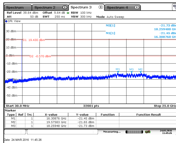
Figure 7.5.1.2-7: 30 MHz – 25 GHz – MCH – u.fl Port
