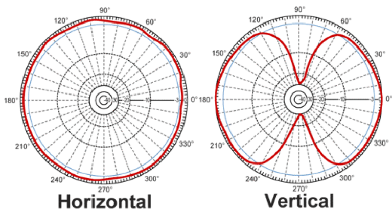
Figure 3: HyperLink Technologies HG2405RD-RSP Antenna Gain Performance
