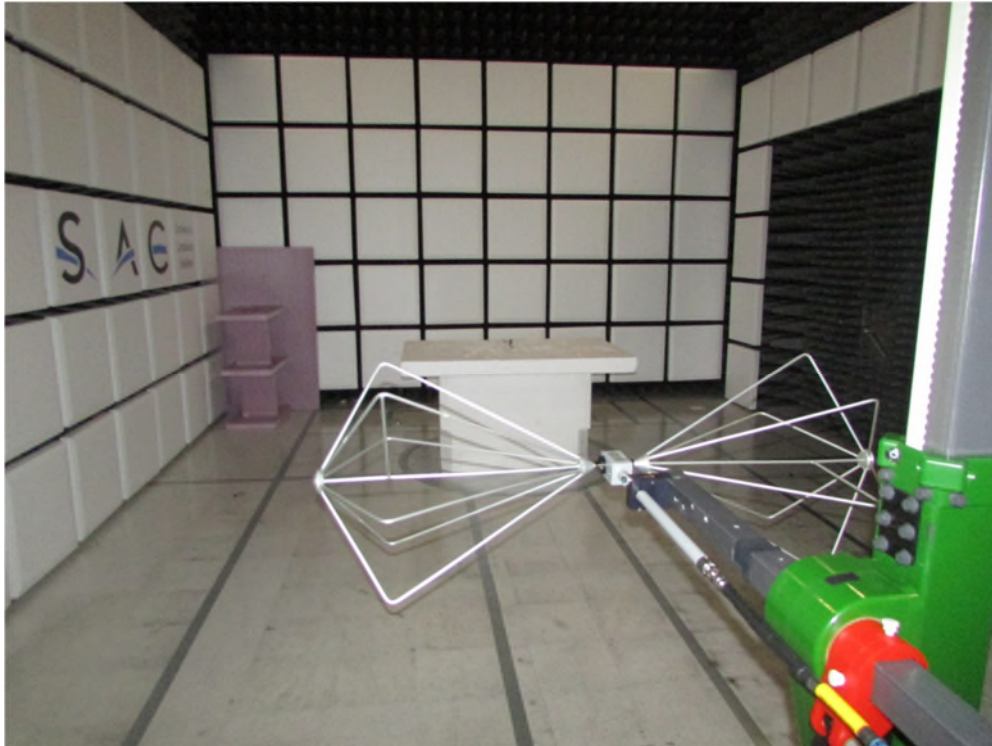
Figure 1: Radiated Emissions – Front – Y-Plane – Below 1GHz
