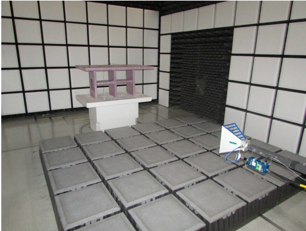
Figure 3: Radiated Emissions – Front – Y-Plane – Above 1GHz
