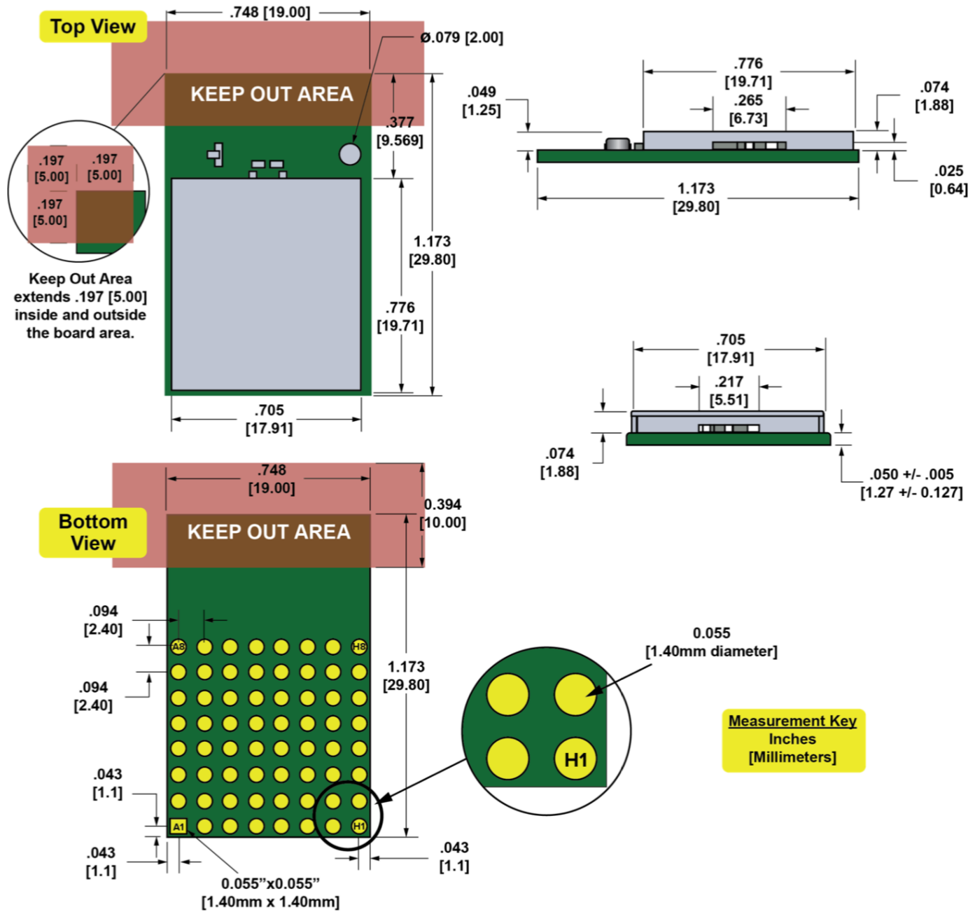
Fig. 1: SM200PF1/PU1 Mechanical Drawing
