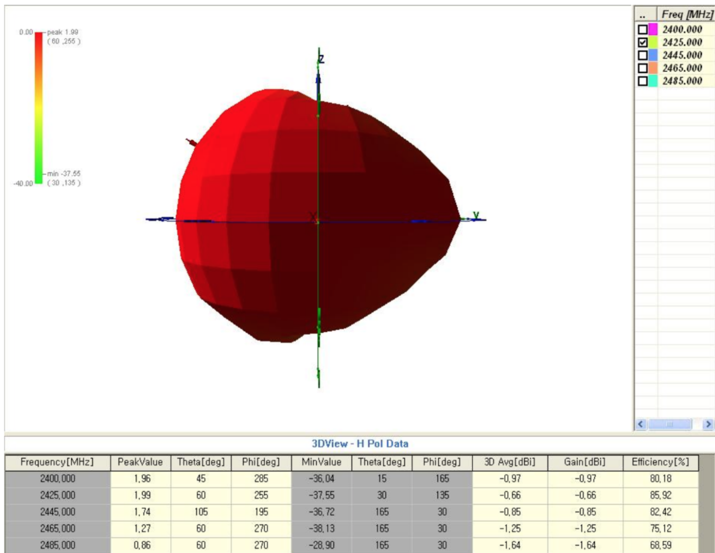
Fig. 1: Partron SDBTPTR3015 Antenna Gain Performance
