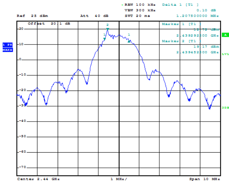
Figure 7.2.2-2: 6dB BW - Middle Channel – RF Port 1
