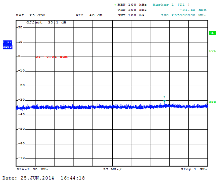
Figure 7.4.2.2-17: 30 MHz – 1 GHz –Middle Channel – RF Port 2
