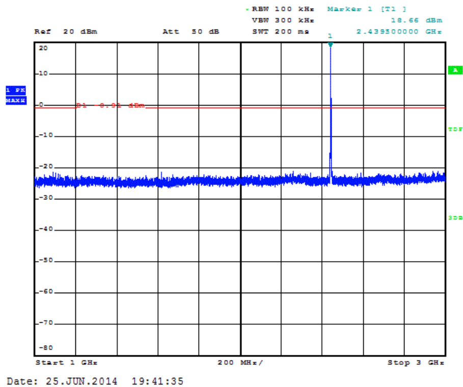
Figure 7.4.2.2-18: 1 GHz – 3 GHz – Middle Channel – RF Port 2
