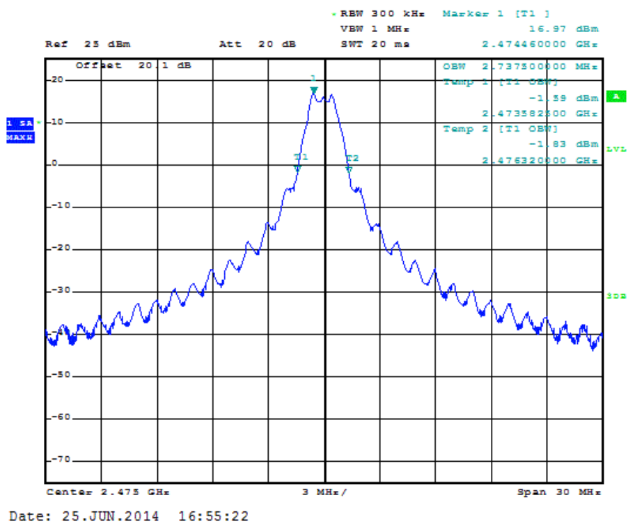
Figure 7.2.2-12: 99% OBW - High Channel – RF Port 2
