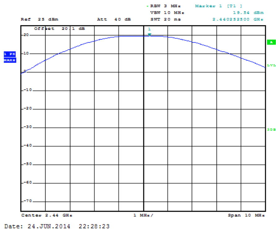
Figure 7.3.2-2: RF Output Power - Middle Channel – RF Port 1
