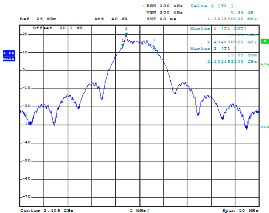
Figure 7.2.2-1: 6dB BW - Low Channel – RF Port 1
