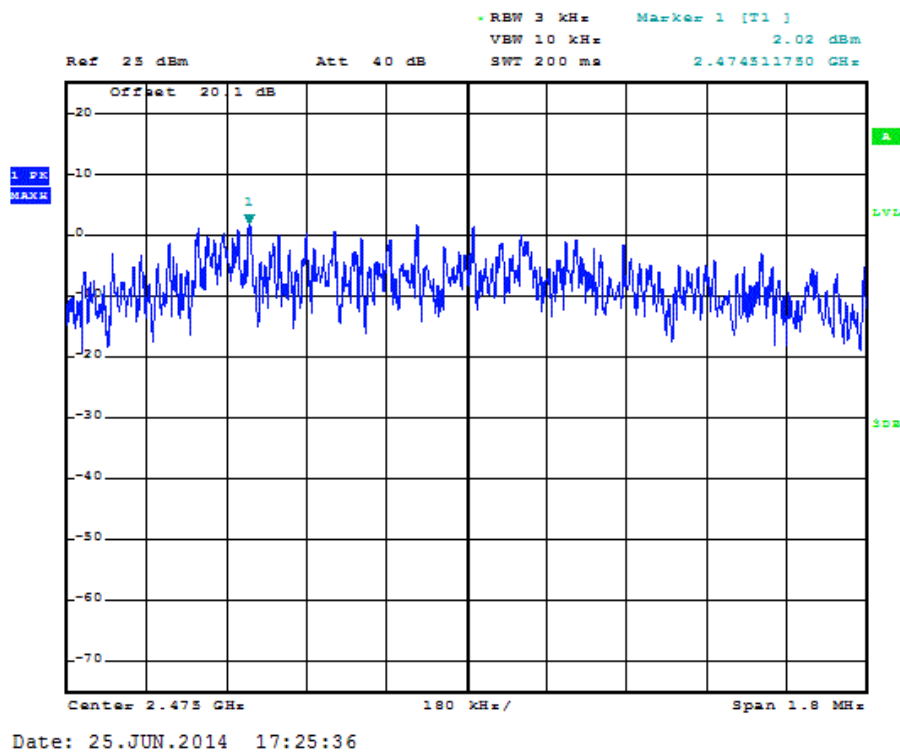
Figure 7.5.2-6: Power Spectral Density – High Channel – RF Port 2
