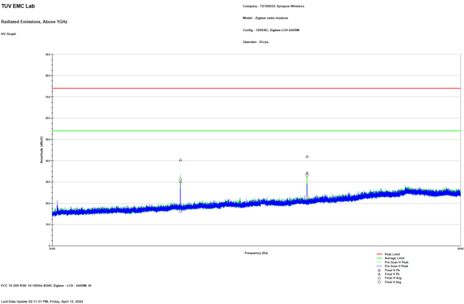
Figure 7: Reference plot for Radiated Spurious Emissions – 10 – 18 GHz– H/V polarity – 2405 MHz
