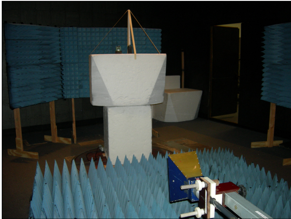
Figure 3: Radiated Emissions – Dipole Antenna YPOS
