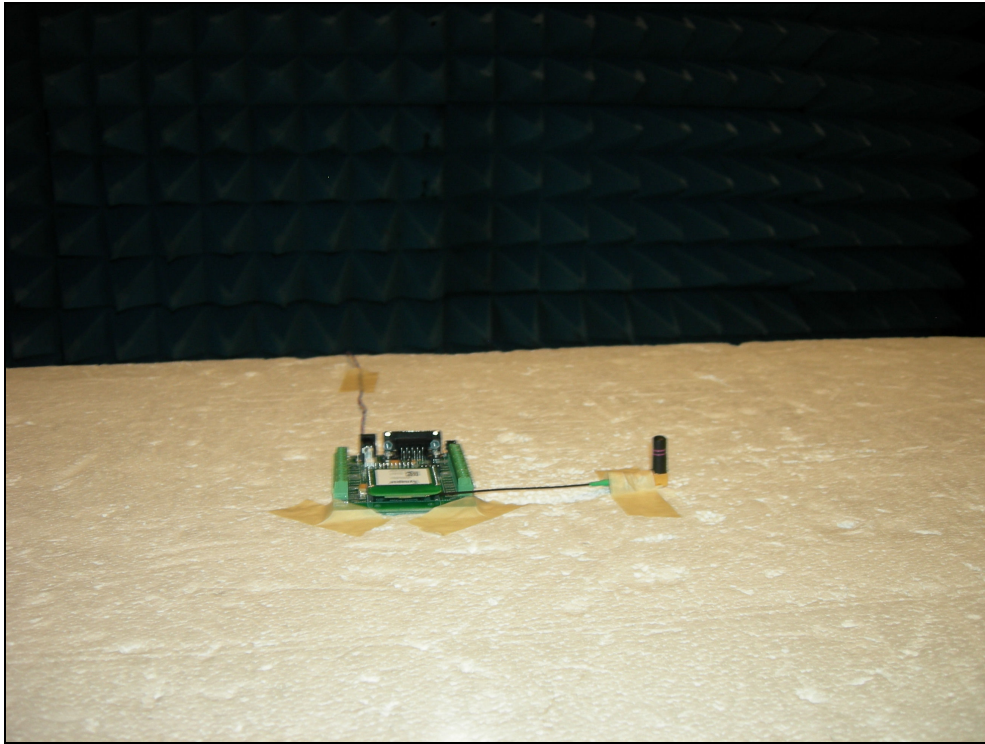
Figure 11: Radiated Emissions – Stubby Antenna ZPOS
