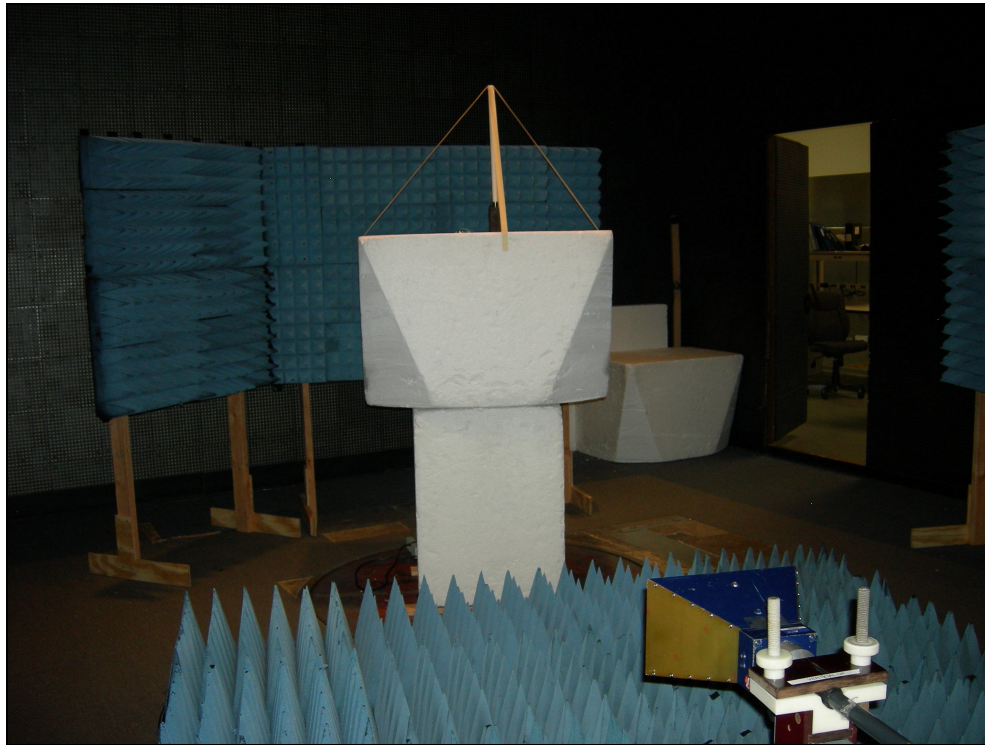
Figure 5: Radiated Emissions – Dipole Antenna ZPOS
