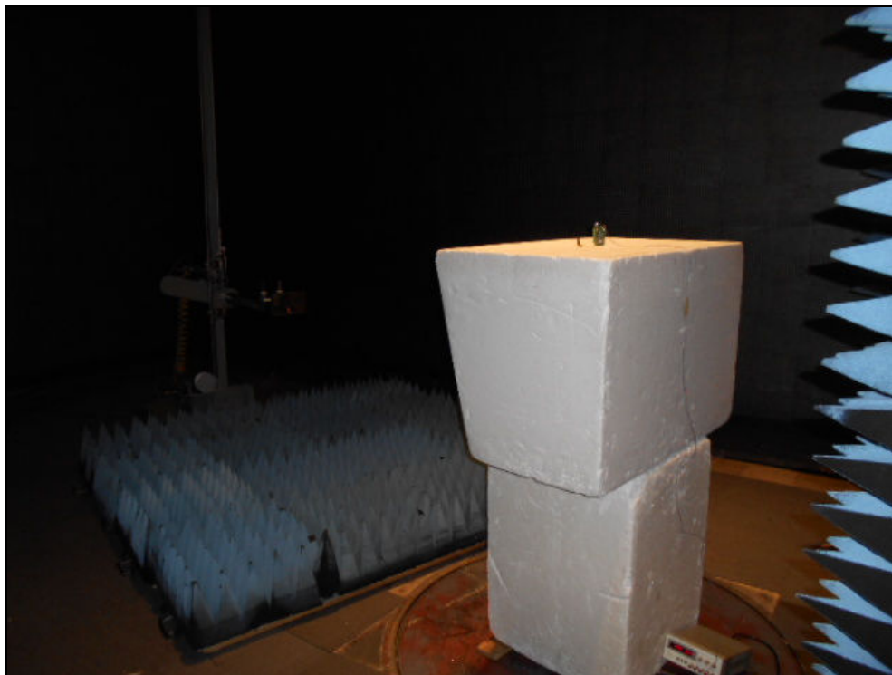
Figure 10: Radiated Emissions – Stubby Antenna YPOS
