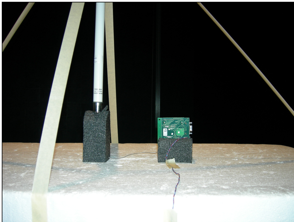
Figure 2: Radiated Emissions – Dipole Antenna XPOS
