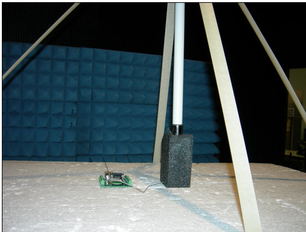
Figure 6: Radiated Emissions – Dipole Antenna ZPOS
