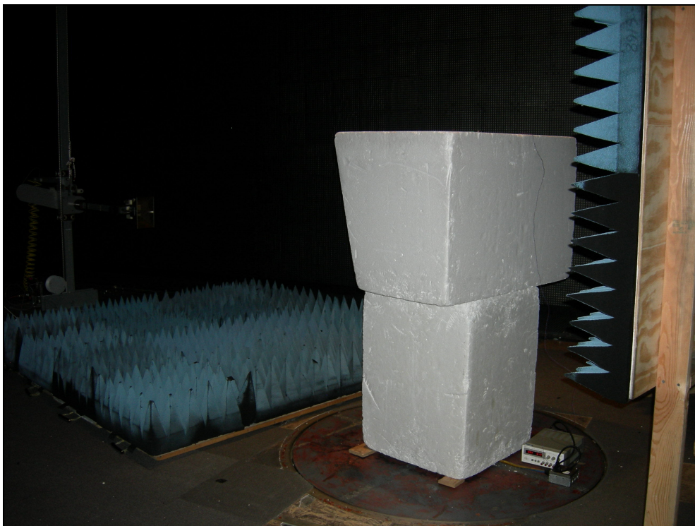
Figure 12: Radiated Emissions – Stubby Antenna ZPOS
