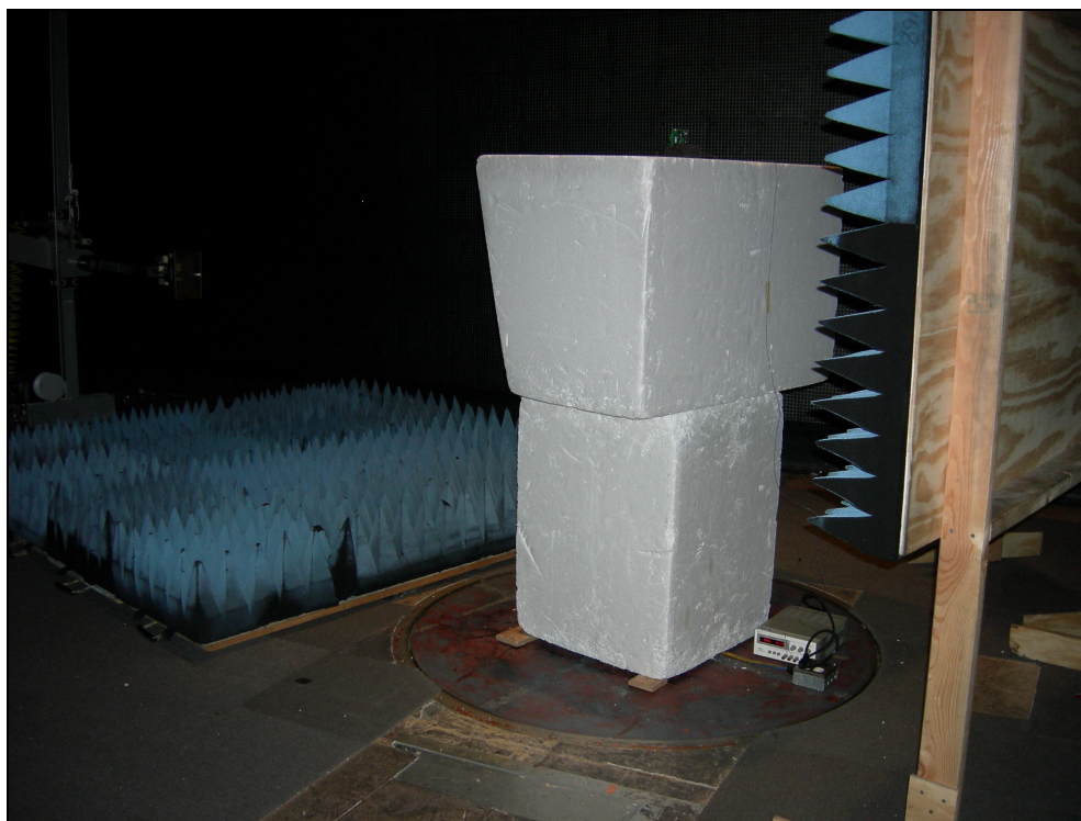
Figure 8: Radiated Emissions – Stubby Antenna XPOS
