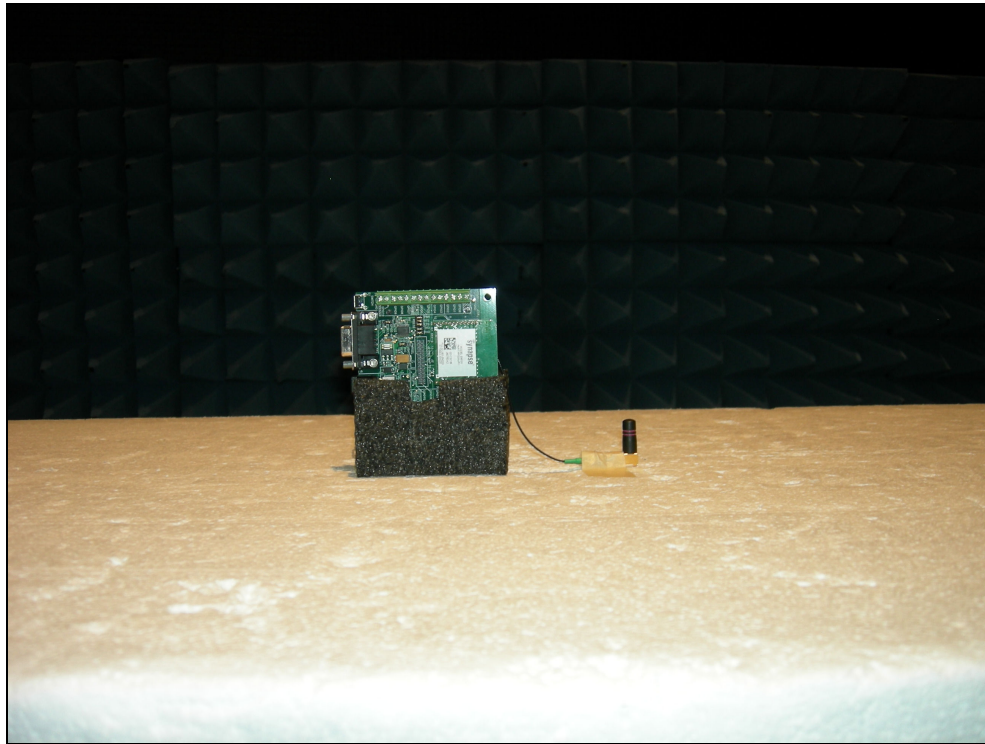
Figure 7: Radiated Emissions – Stubby Antenna XPOS
