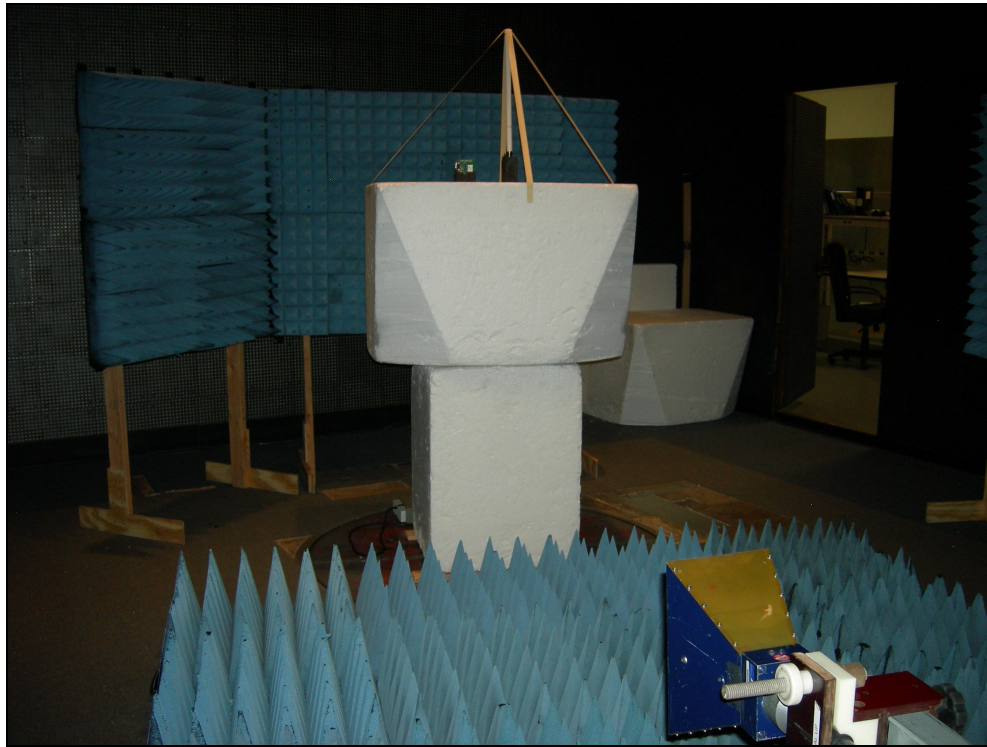
Figure 1: Radiated Emissions – Dipole Antenna XPOS
