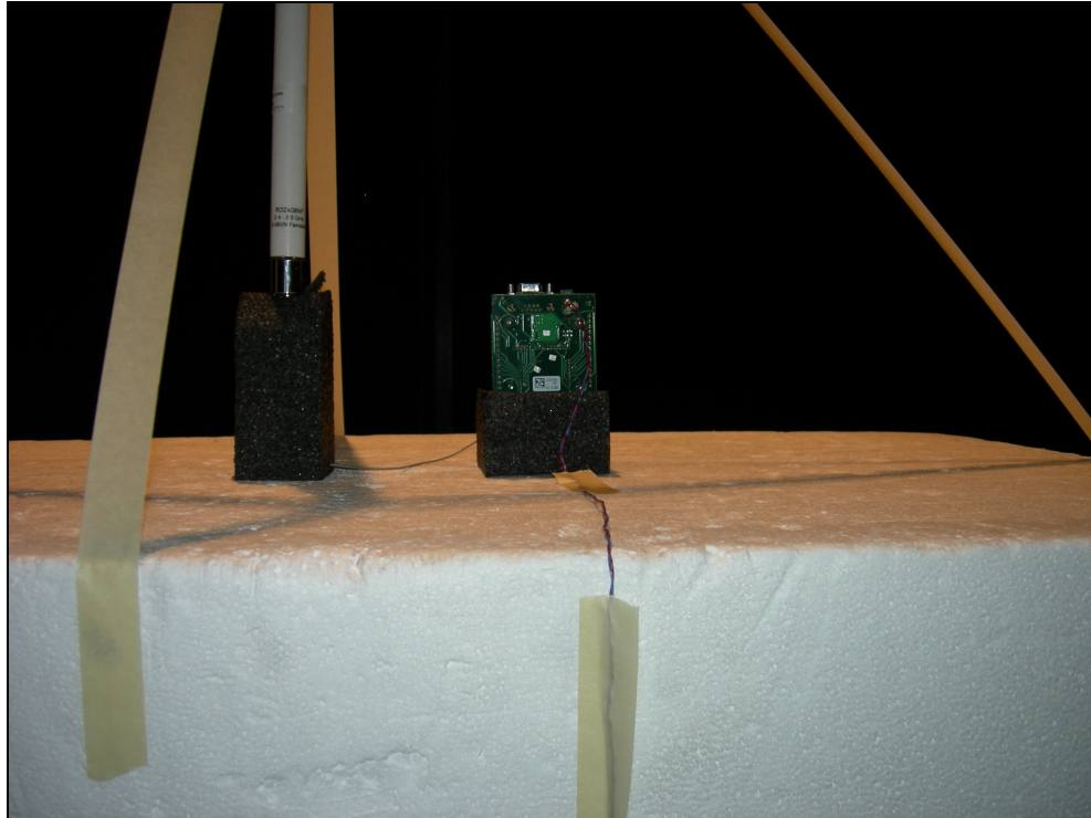
Figure 4: Radiated Emissions – Dipole Antenna YPOS
