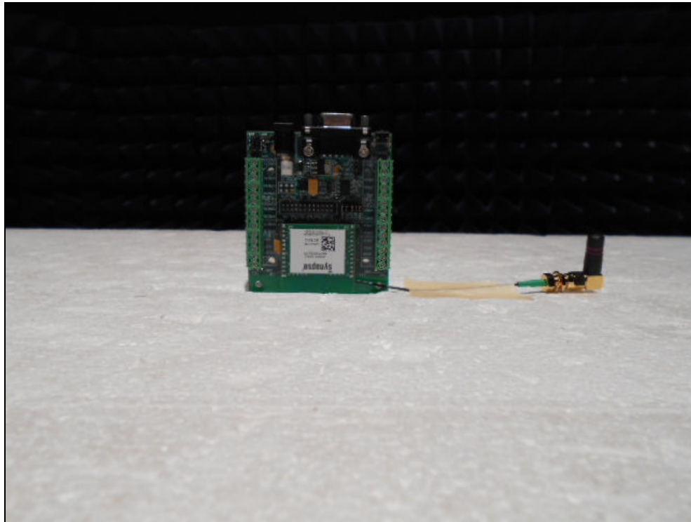
Figure 9: Radiated Emissions – Stubby Antenna YPOS
