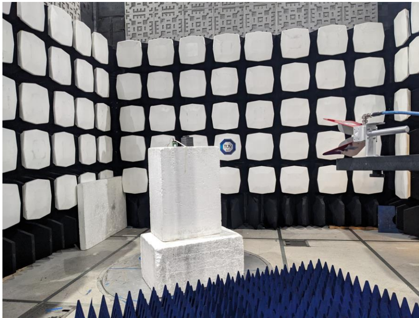
Figure:5– Test Set up – Front View of the EUT - Radiated Emissions <10 GHz
