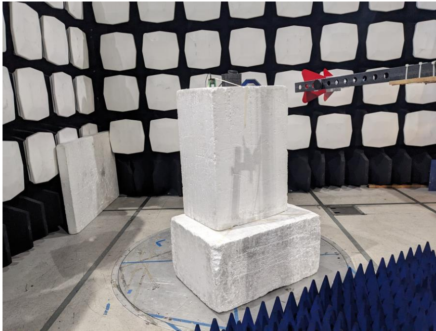
Figure:7– Test Set up – Front View of the EUT - Radiated Emissions <18 GHz
