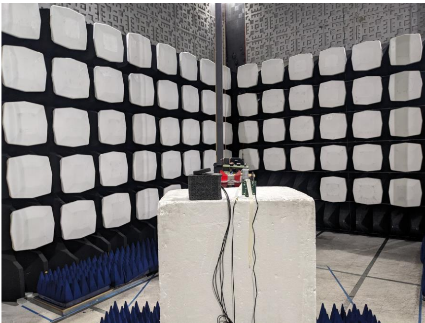
Figure:8– Test Set up – Rear View of the EUT - Radiated Emissions <18 GHz
