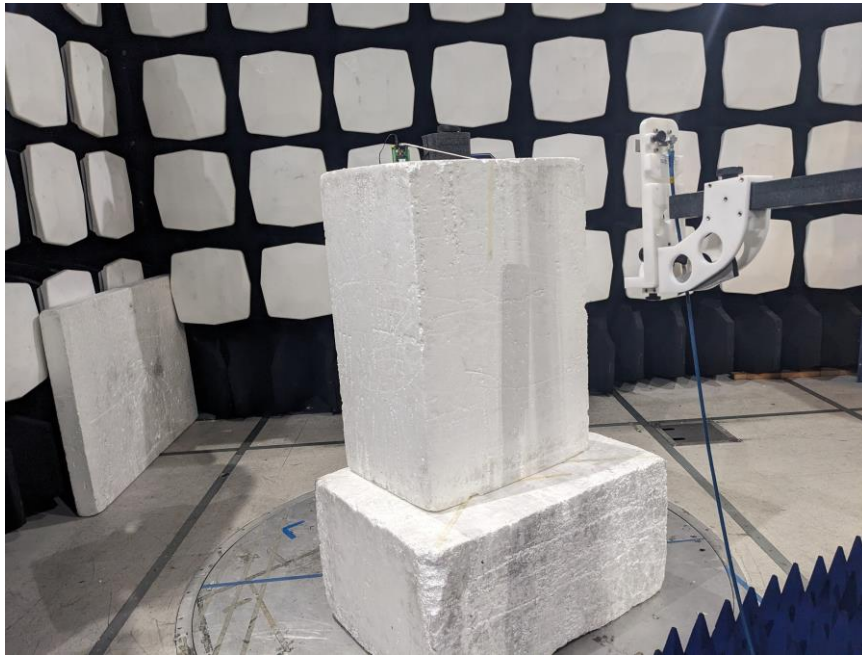
Figure:9– Test Set up – Front View of the EUT - Radiated Emissions <26 GHz
