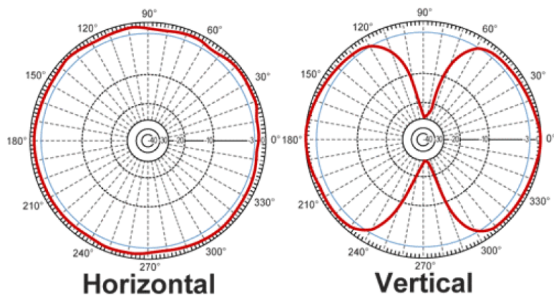
Figure 3: HyperLink Technologies HG2405RD-RSP Antenna Gain Performance
