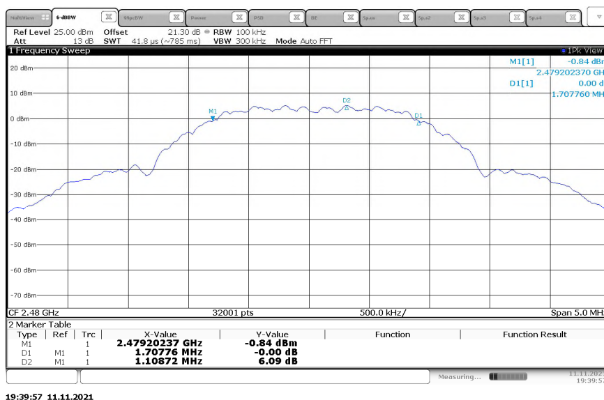
Figure 2.2.6-3: 6 dB Bandwidth Test Results High Channel
