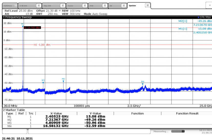
Figure 2.6.6-1: RF Conducted Spurious Emissions Results Low Channel
