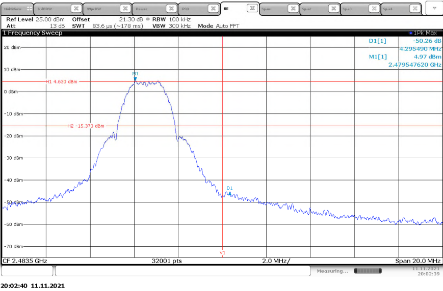
Figure 2.5.6-2: RF Conducted Band-Edge Results High Channel
