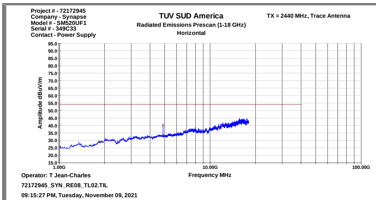
Figure 2.8.7-4: Radiated Emissions Representative Scan 1 GHz – 18 GHz Horizontal Polarization – Trace Antenna
