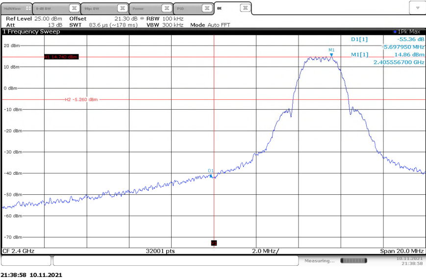
Figure 2.5.6-1: RF Conducted Band-Edge Results Low Channel
