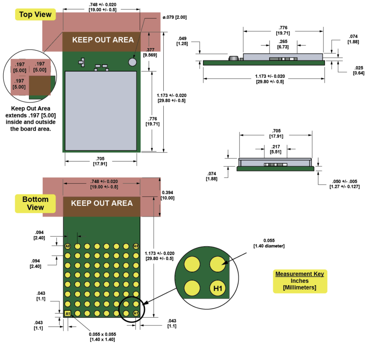
Fig. 1: SM520UF1 Mechanical Drawing
