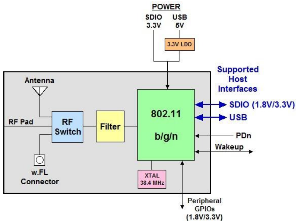
Figure 1: Block Diagram
