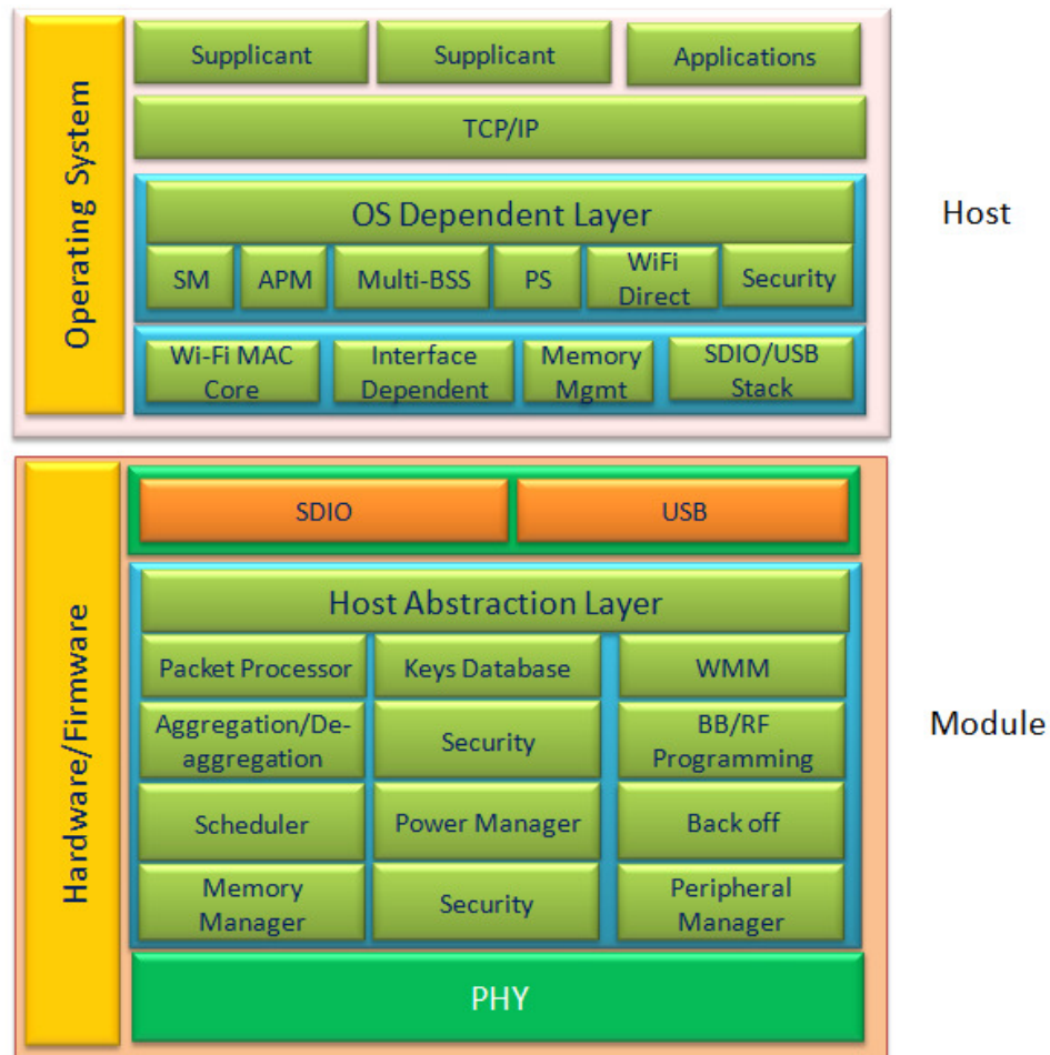
Figure 5: Stack Diagram
