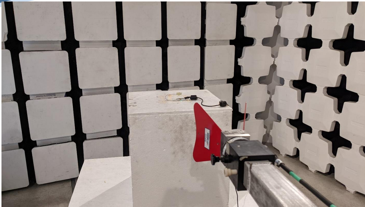
Dual Patch
