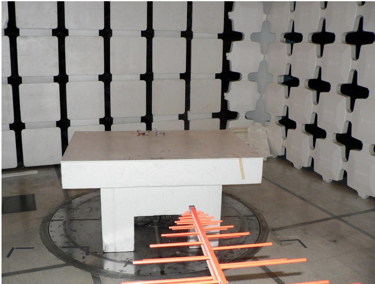
AL5808_Octal Digital Emissions 30-1000MHz
