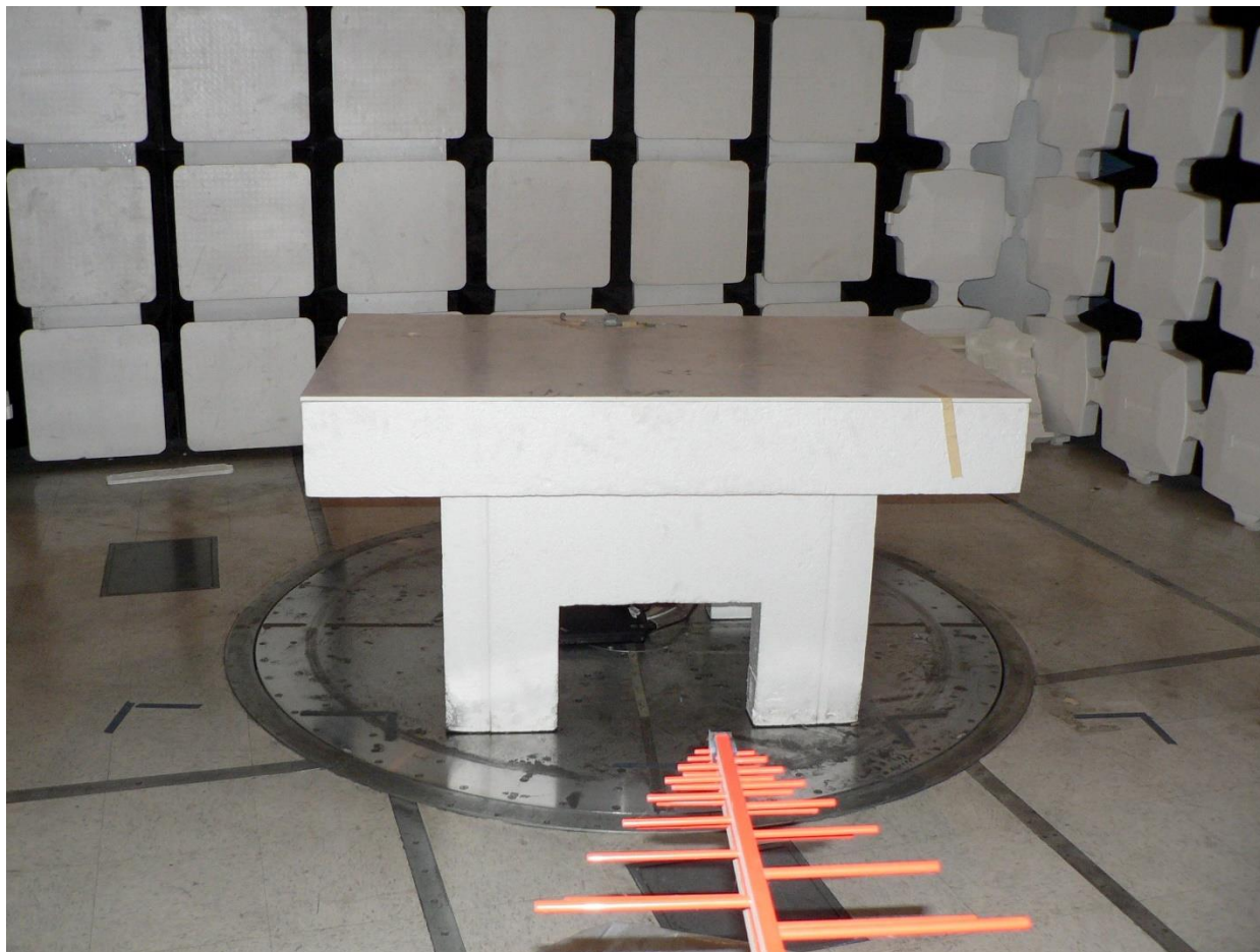
AL5834_Combat256 Digital Emissions 30-1000MHz
