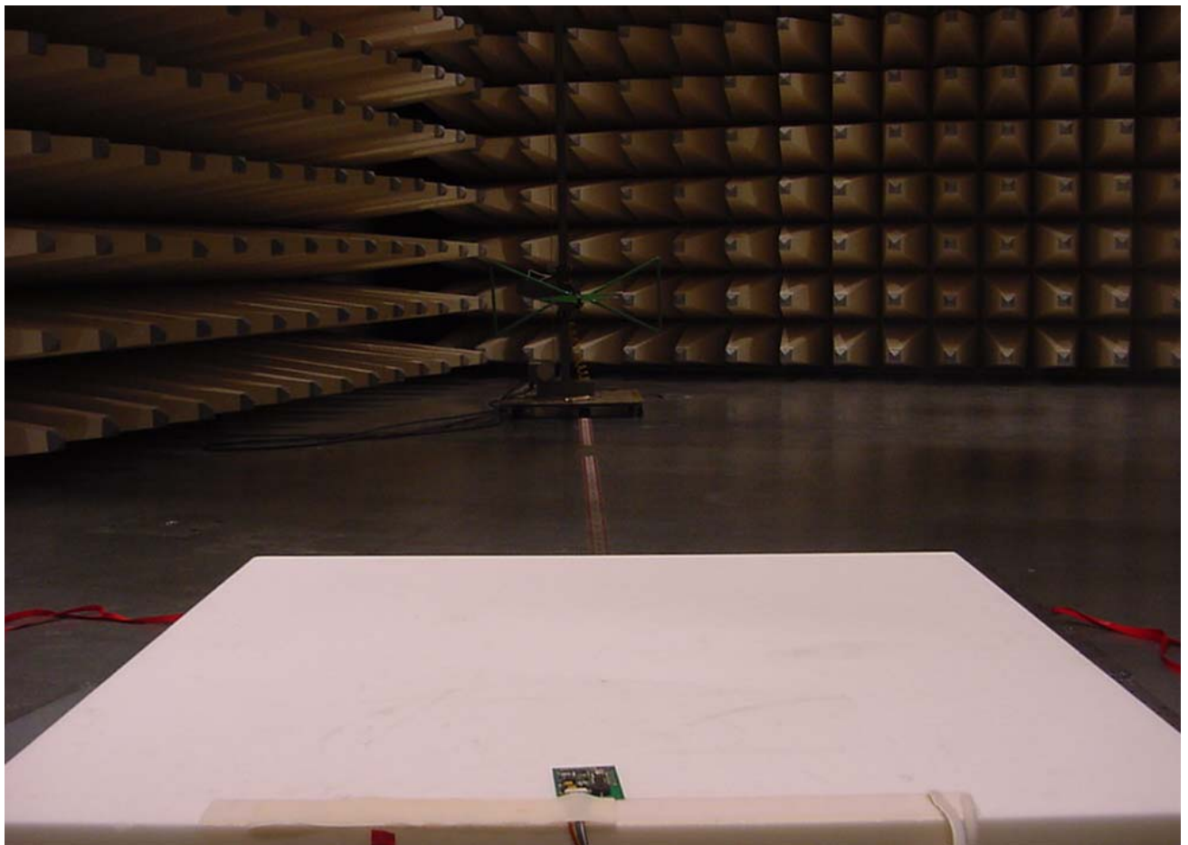
Photo 1 (Radiated Emissions):
