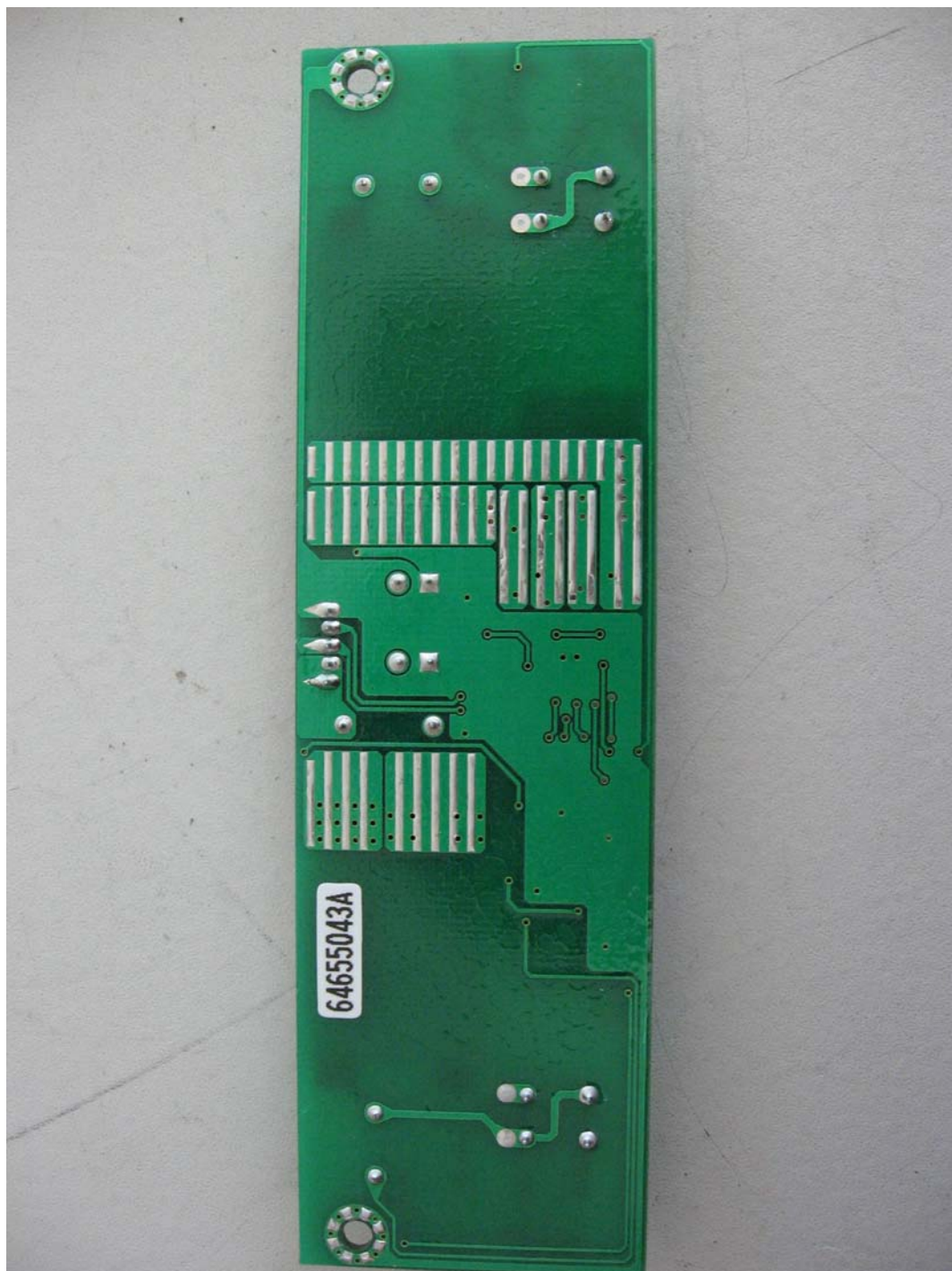
Inverter Board Rear
