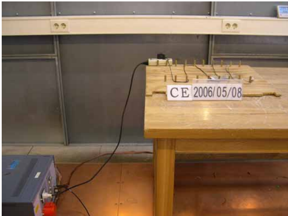
Fig C.1 Conducted Emission
