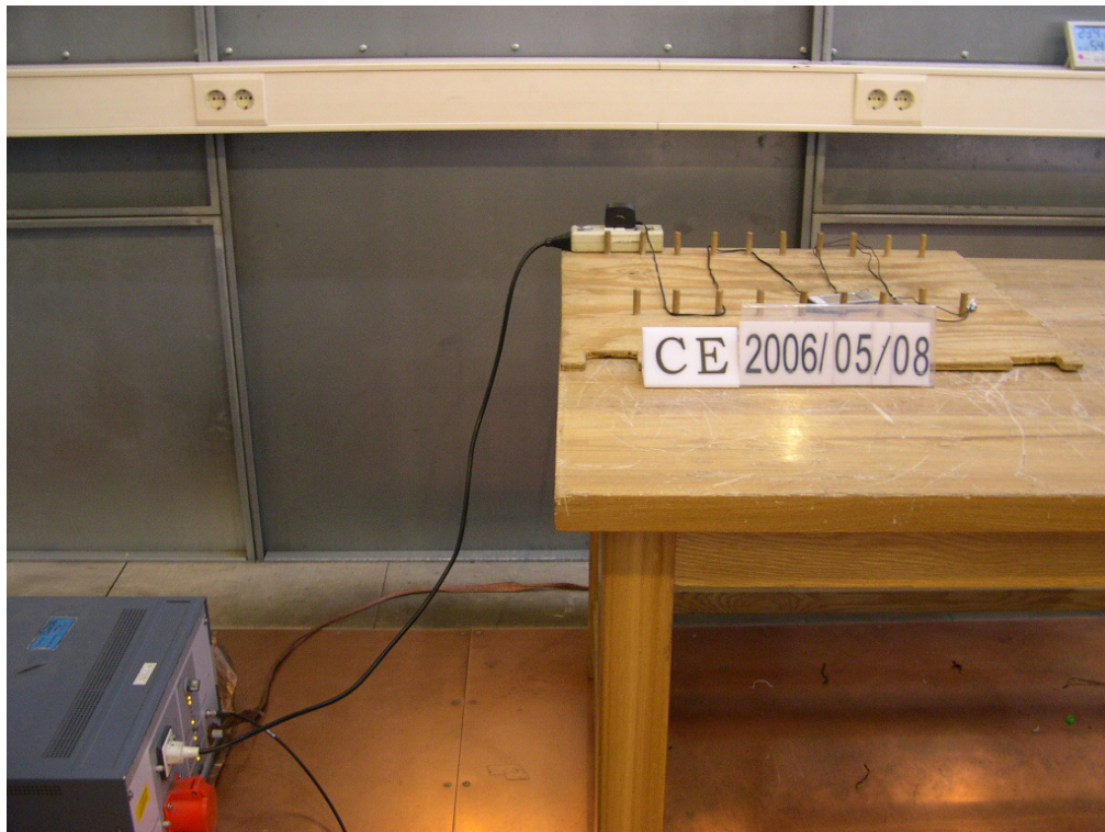
Fig C.1 Conducted Emission
