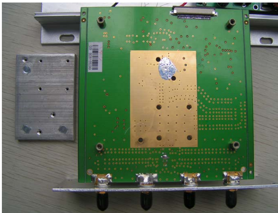
Main Board #1 Screw Holder Removed Rear View
