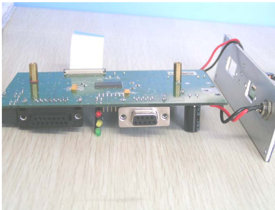
Main Board #2 Side Connector View
