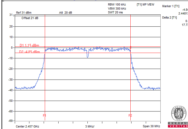
802.11n (HT20): Chain 1 / CH10
