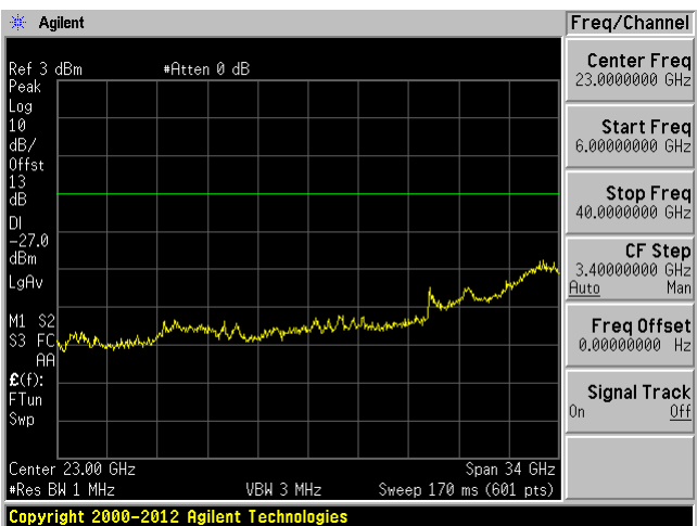
Middle 5200 MHz (6GHz – 40GHz)
