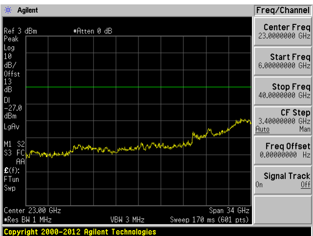
802.11a Middle 5200 MHz (6-40GHz)
