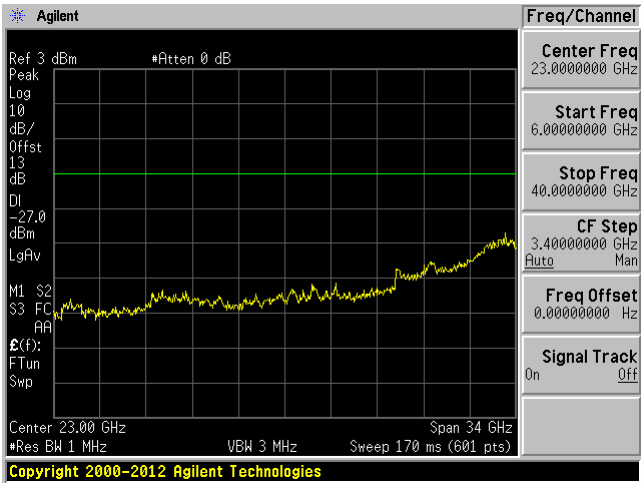
802.11a High 5240 MHz (6-40GHz)
