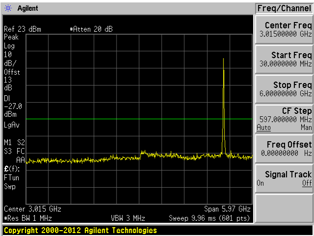
802.11a High 5240MHz (30MHz-6GHz)
