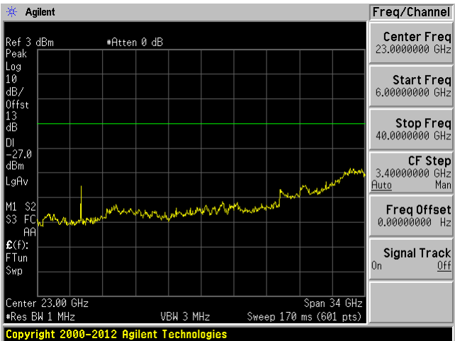
802.11n20 Low 5190 MHz (6-40GHz)
