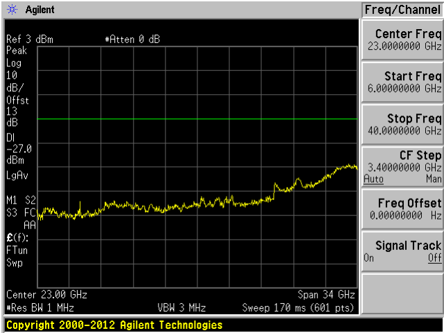
802.11n20 Low 5180 MHz (6-40GHz)
