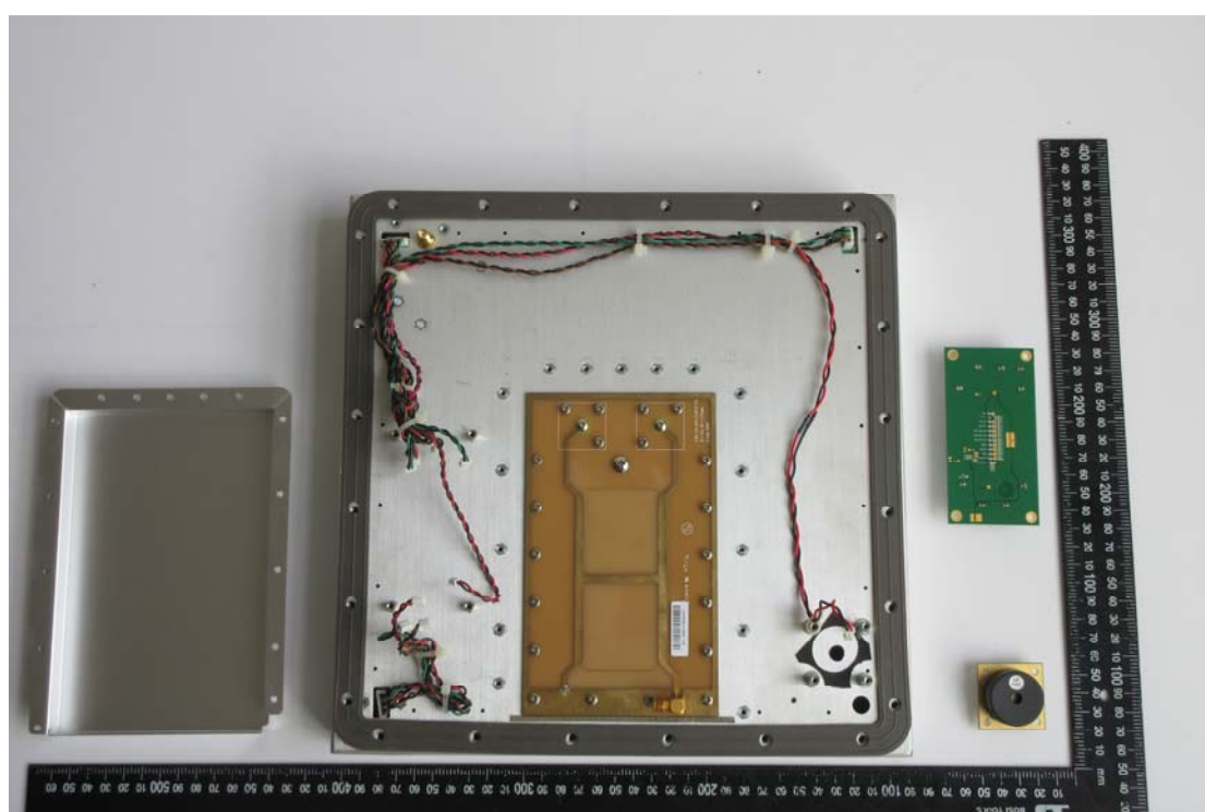
7. RFID antenna view
