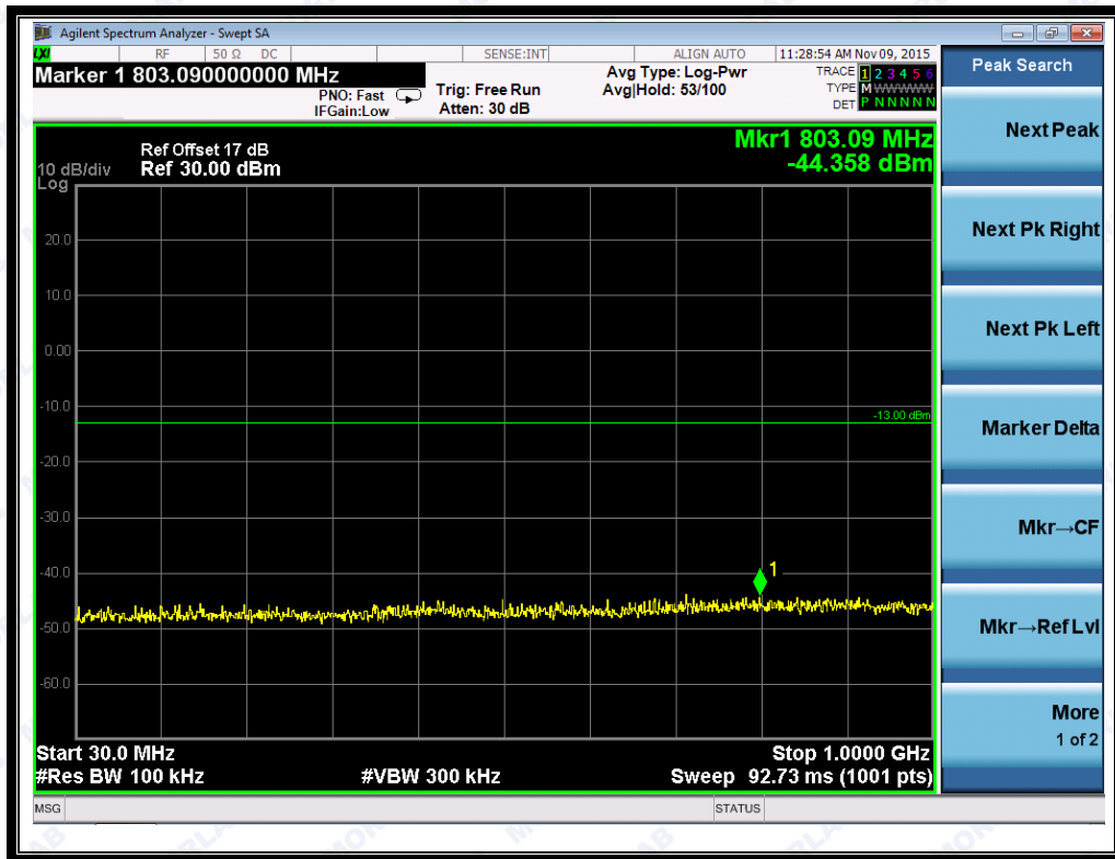
(Plot J3: HSUPA1700MHz Channel = 1513, 30MHz to 1GHz)
